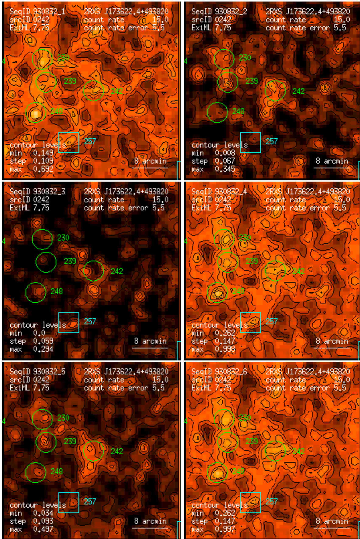
Figure 242: RASS 930832: detection 0242: band rate images, Gaussian filter: (1) PSPC channels 11 – 41, (2) 52 – 90, (3) 91 – 201, (4) 11 – 235, (5) 52 – 201, (6) 11 – 201. Broad band rates in counts/ks. Band rate contour levels in counts/ks/arcmin 2 .
