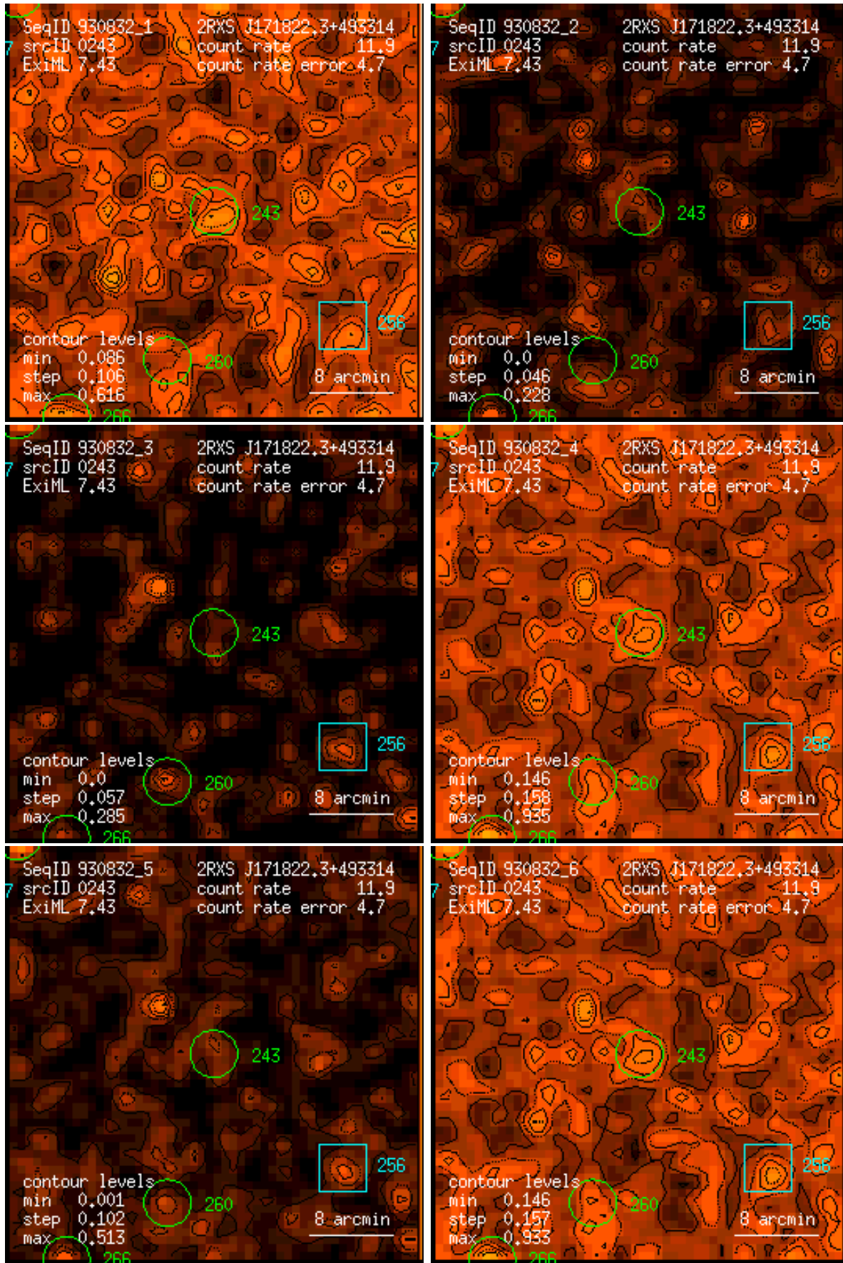
Figure 243: RASS 930832: detection 0243: band rate images, Gaussian filter: (1) PSPC channels 11 – 41, (2) 52 – 90, (3) 91 – 201, (4) 11 – 235, (5) 52 – 201, (6) 11 – 201. Broad band rates in counts/ks. Band rate contour levels in counts/ks/arcmin 2 .
