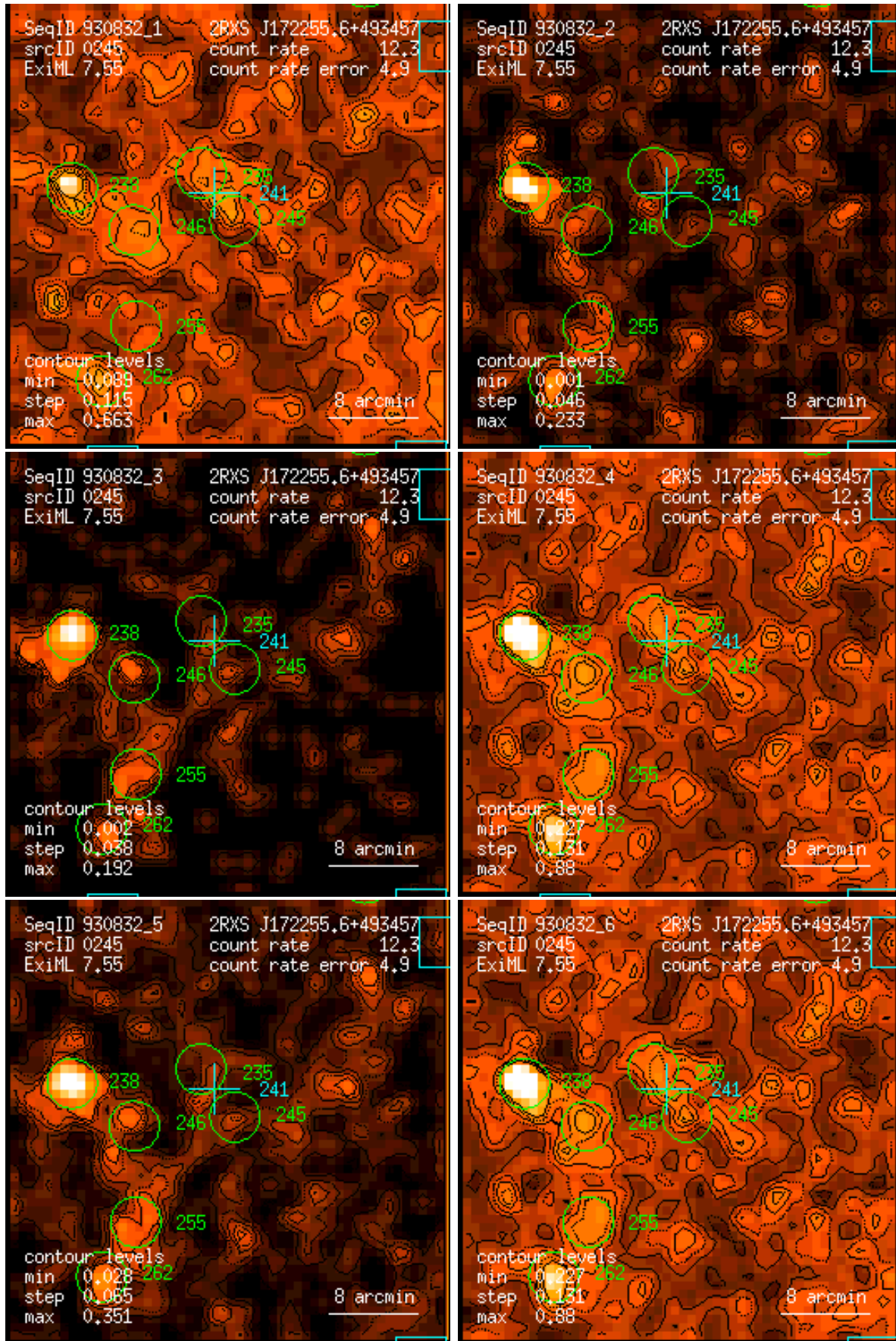
Figure 245: RASS 930832: detection 0245: band rate images, Gaussian filter: (1) PSPC channels 11 – 41, (2) 52 – 90, (3) 91 – 201, (4) 11 – 235, (5) 52 – 201, (6) 11 – 201. Broad band rates in counts/ks. Band rate contour levels in counts/ks/arcmin 2 .
