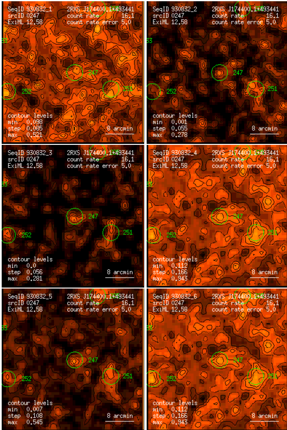
Figure 247: RASS 930832: detection 0247: band rate images, Gaussian filter: (1) PSPC channels 11 – 41, (2) 52 – 90, (3) 91 – 201, (4) 11 – 235, (5) 52 – 201, (6) 11 – 201. Broad band rates in counts/ks. Band rate contour levels in counts/ks/arcmin 2 .
