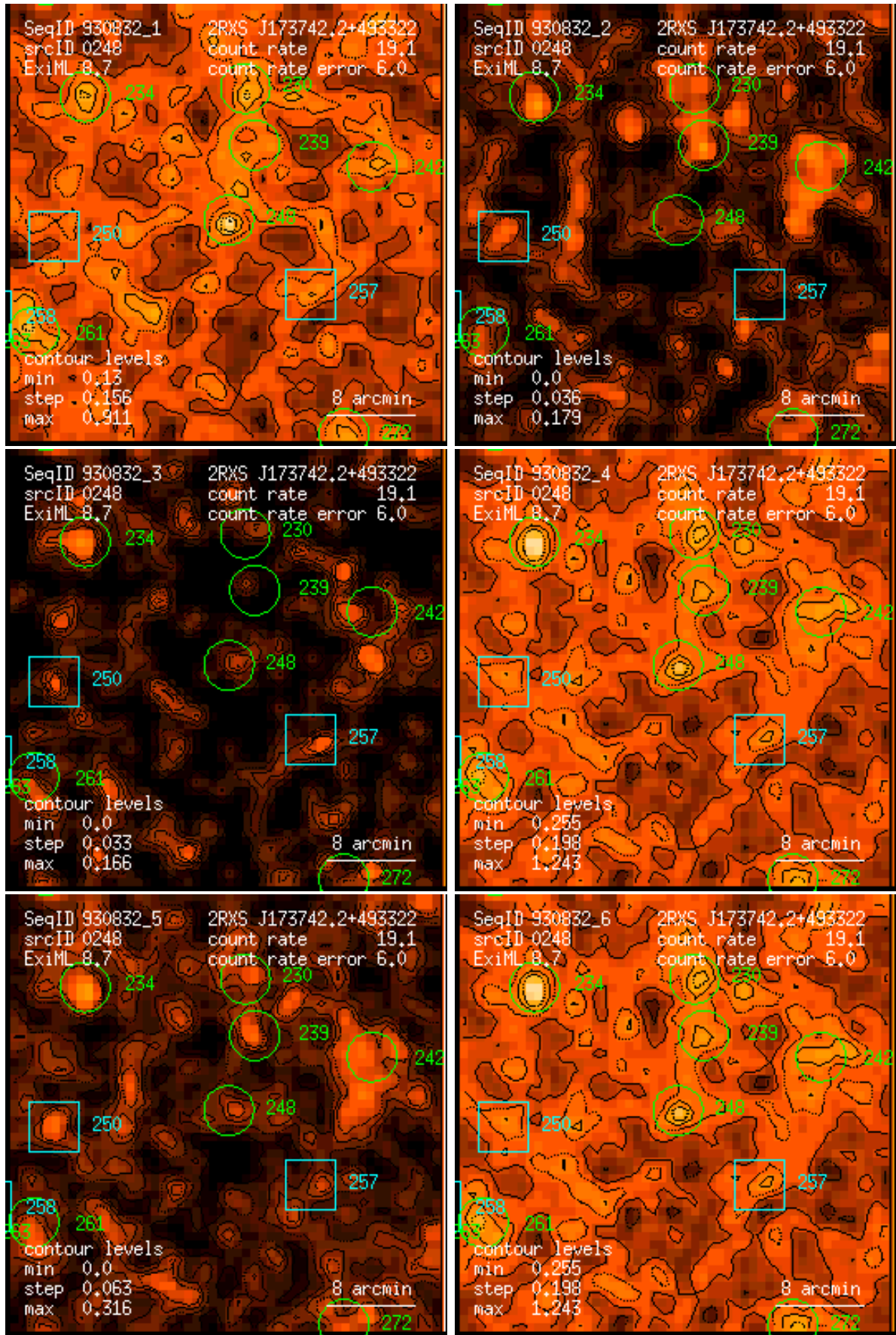
Figure 248: RASS 930832: detection 0248: band rate images, Gaussian filter: (1) PSPC channels 11 – 41, (2) 52 – 90, (3) 91 – 201, (4) 11 – 235, (5) 52 – 201, (6) 11 – 201. Broad band rates in counts/ks. Band rate contour levels in counts/ks/arcmin 2 .
