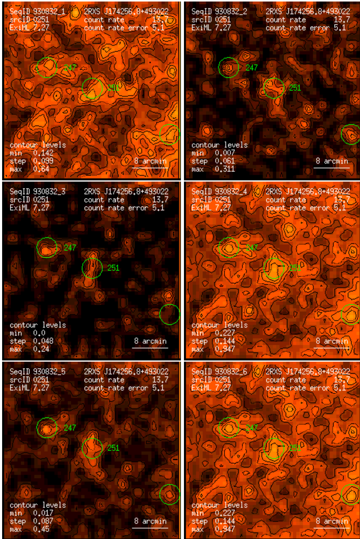
Figure 251: RASS 930832: detection 0251: band rate images, Gaussian filter: (1) PSPC channels 11 – 41, (2) 52 – 90, (3) 91 – 201, (4) 11 – 235, (5) 52 – 201, (6) 11 – 201. Broad band rates in counts/ks. Band rate contour levels in counts/ks/arcmin 2 .
