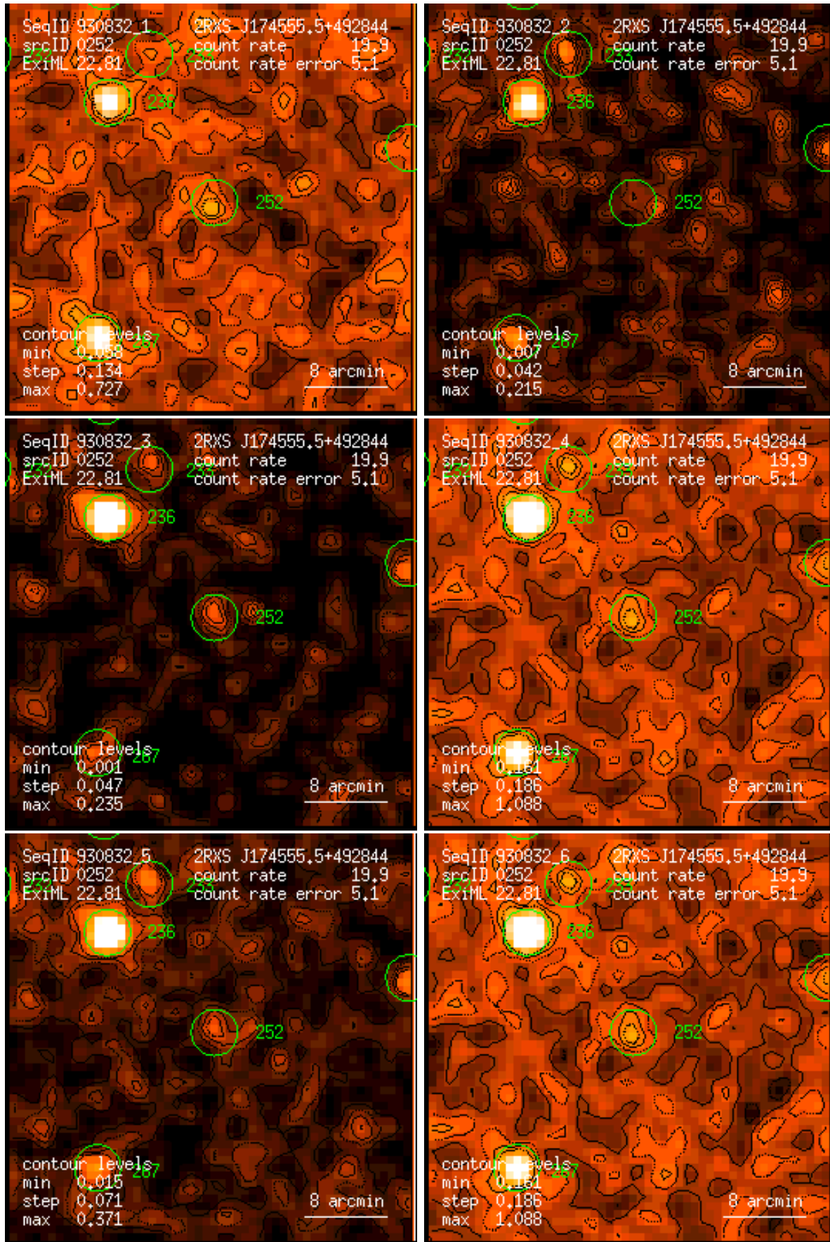
Figure 252: RASS 930832: detection 0252: band rate images, Gaussian filter: (1) PSPC channels 11 – 41, (2) 52 – 90, (3) 91 – 201, (4) 11 – 235, (5) 52 – 201, (6) 11 – 201. Broad band rates in counts/ks. Band rate contour levels in counts/ks/arcmin 2 .
