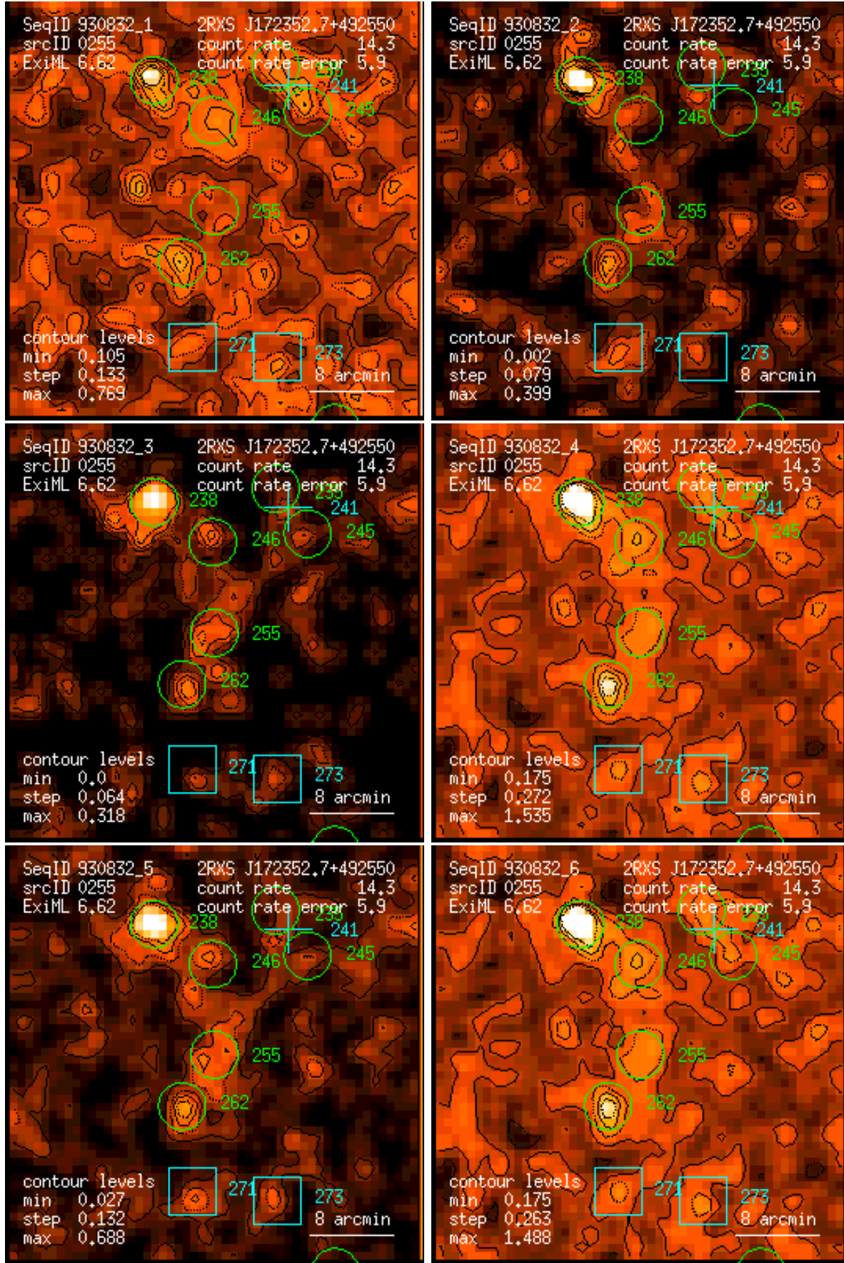
Figure 255: RASS 930832: detection 0255: band rate images, Gaussian filter: (1) PSPC channels 11 – 41, (2) 52 – 90, (3) 91 – 201, (4) 11 – 235, (5) 52 – 201, (6) 11 – 201. Broad band rates in counts/ks. Band rate contour levels in counts/ks/arcmin 2 .
