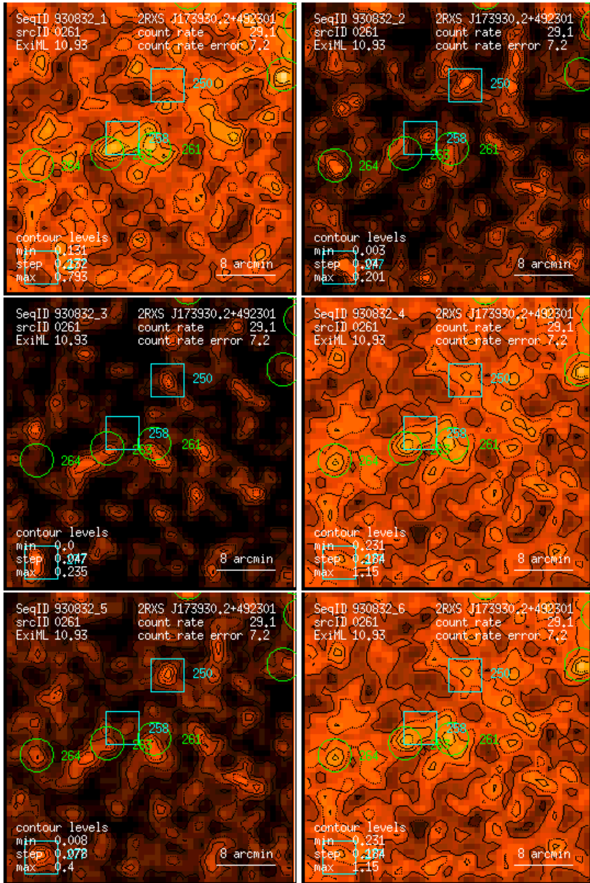
Figure 261: RASS 930832: detection 0261: band rate images, Gaussian filter: (1) PSPC channels 11 – 41, (2) 52 – 90, (3) 91 – 201, (4) 11 – 235, (5) 52 – 201, (6) 11 – 201. Broad band rates in counts/ks. Band rate contour levels in counts/ks/arcmin 2 .
