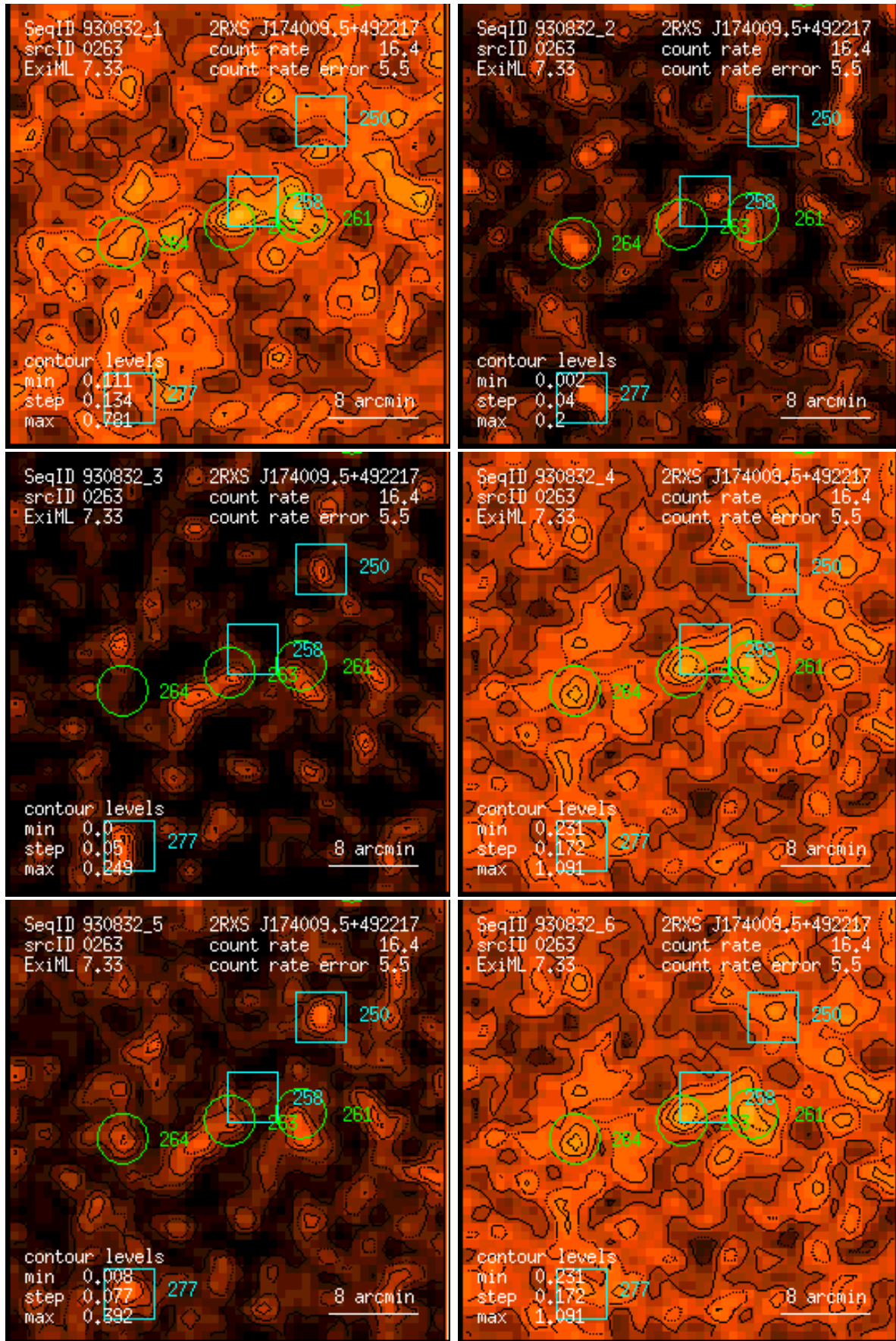
Figure 263: RASS 930832: detection 0263: band rate images, Gaussian filter: (1) PSPC channels 11 – 41, (2) 52 – 90, (3) 91 – 201, (4) 11 – 235, (5) 52 – 201, (6) 11 – 201. Broad band rates in counts/ks. Band rate contour levels in counts/ks/arcmin 2 .
