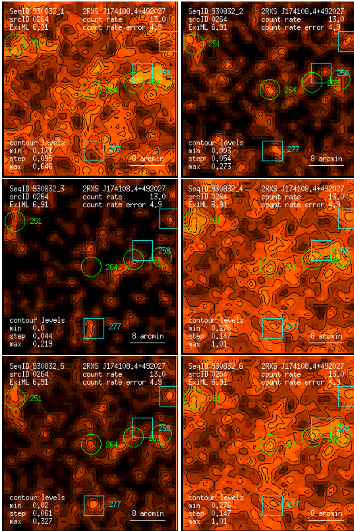
Figure 264: RASS 930832: detection 0264: band rate images, Gaussian filter: (1) PSPC channels 11 – 41, (2) 52 – 90, (3) 91 – 201, (4) 11 – 235, (5) 52 – 201, (6) 11 – 201. Broad band rates in counts/ks. Band rate contour levels in counts/ks/arcmin 2 .
