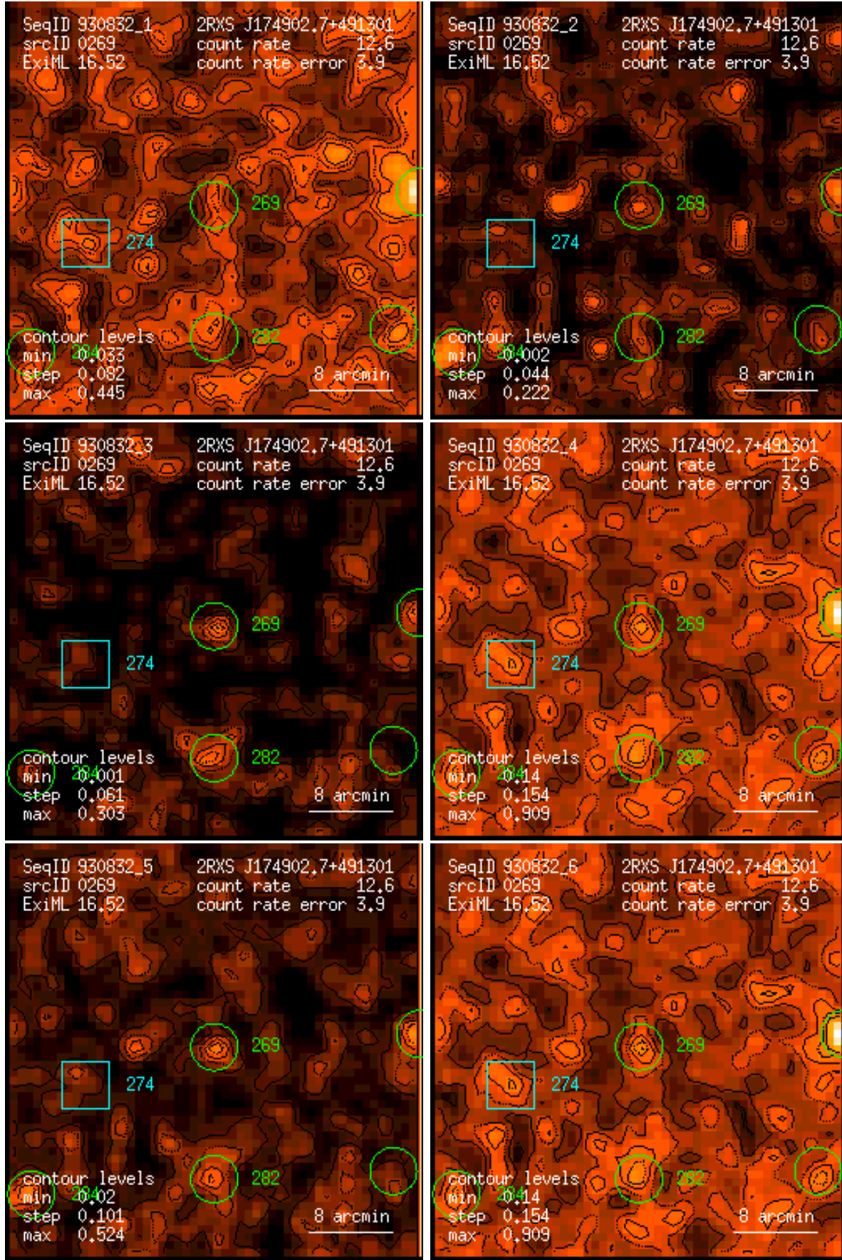
Figure 269: RASS 930832: detection 0269: band rate images, Gaussian filter: (1) PSPC channels 11 – 41, (2) 52 – 90, (3) 91 – 201, (4) 11 – 235, (5) 52 – 201, (6) 11 – 201. Broad band rates in counts/ks. Band rate contour levels in counts/ks/arcmin 2 .
