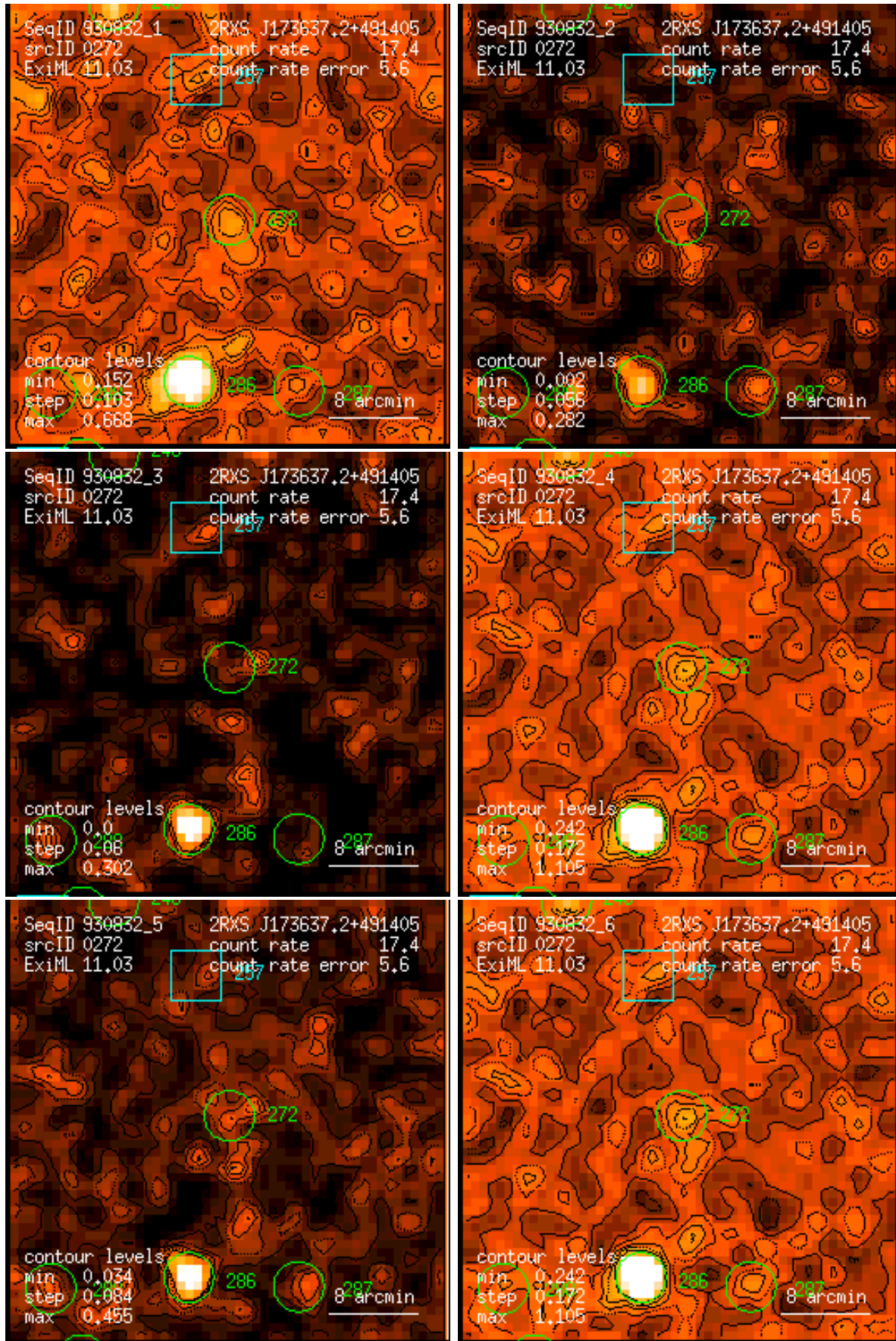
Figure 272: RASS 930832: detection 0272: band rate images, Gaussian filter: (1) PSPC channels 11 – 41, (2) 52 – 90, (3) 91 – 201, (4) 11 – 235, (5) 52 – 201, (6) 11 – 201. Broad band rates in counts/ks. Band rate contour levels in counts/ks/arcmin 2 .
