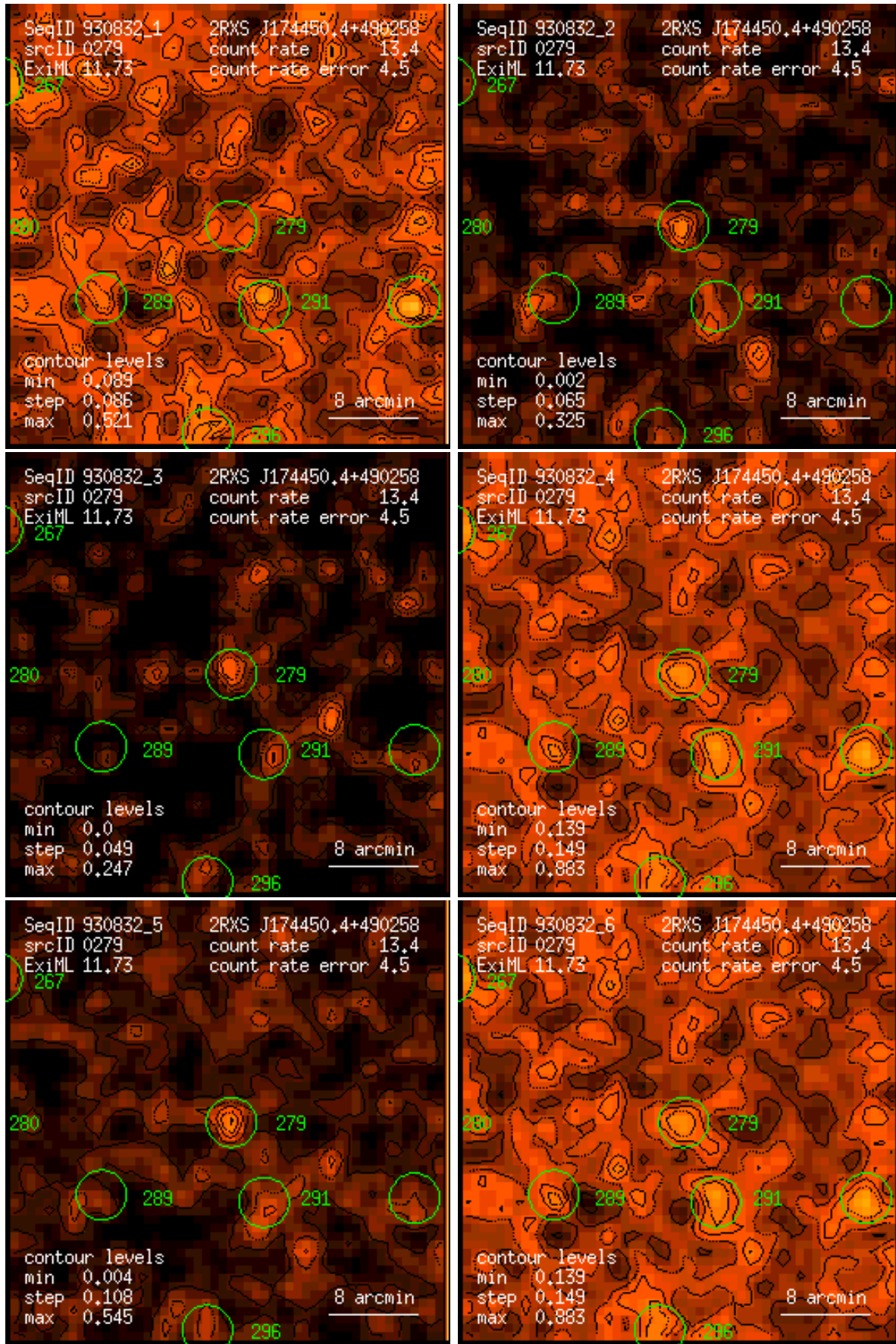
Figure 279: RASS 930832: detection 0279: band rate images, Gaussian filter: (1) PSPC channels 11 – 41, (2) 52 – 90, (3) 91 – 201, (4) 11 – 235, (5) 52 – 201, (6) 11 – 201. Broad band rates in counts/ks. Band rate contour levels in counts/ks/arcmin 2 .
