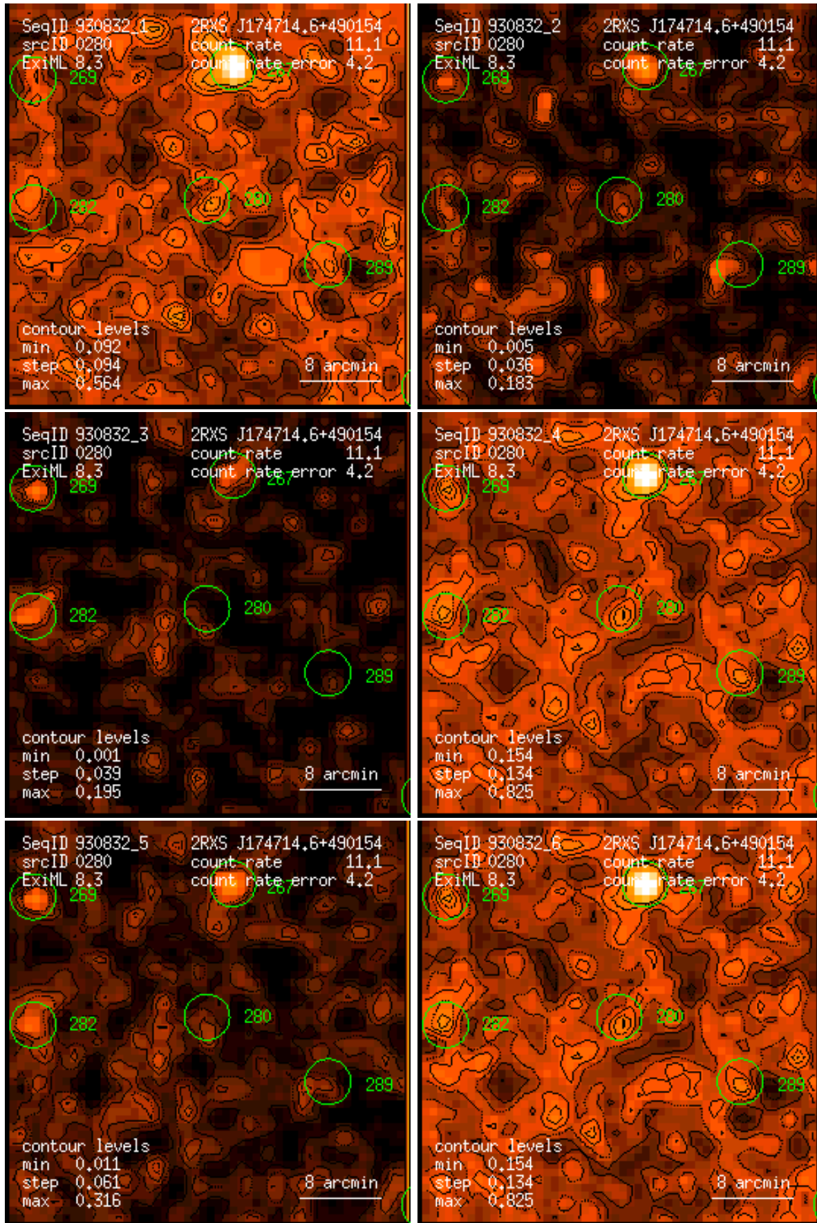
Figure 280: RASS 930832: detection 0280: band rate images, Gaussian filter: (1) PSPC channels 11 – 41, (2) 52 – 90, (3) 91 – 201, (4) 11 – 235, (5) 52 – 201, (6) 11 – 201. Broad band rates in counts/ks. Band rate contour levels in counts/ks/arcmin 2 .
