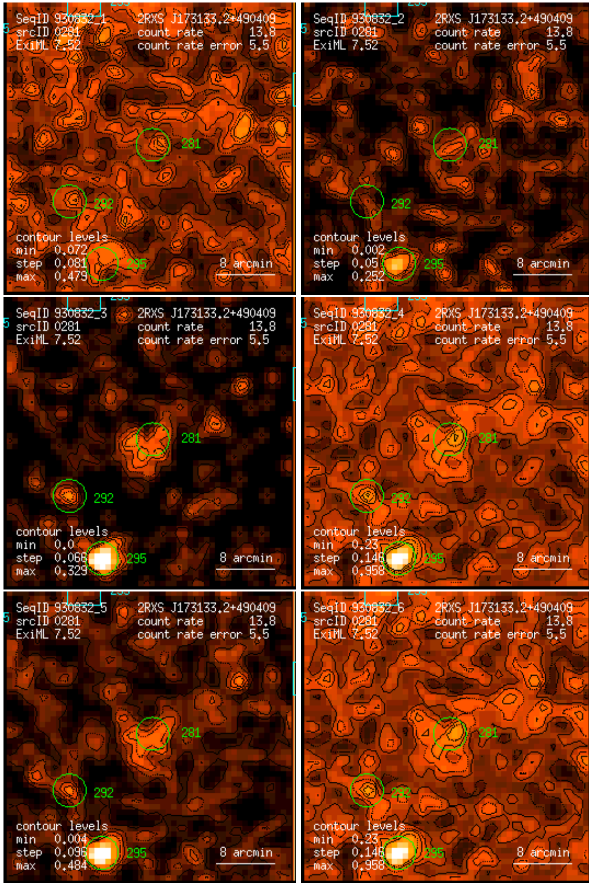
Figure 281: RASS 930832: detection 0281: band rate images, Gaussian filter: (1) PSPC channels 11 – 41, (2) 52 – 90, (3) 91 – 201, (4) 11 – 235, (5) 52 – 201, (6) 11 – 201. Broad band rates in counts/ks. Band rate contour levels in counts/ks/arcmin 2 .
