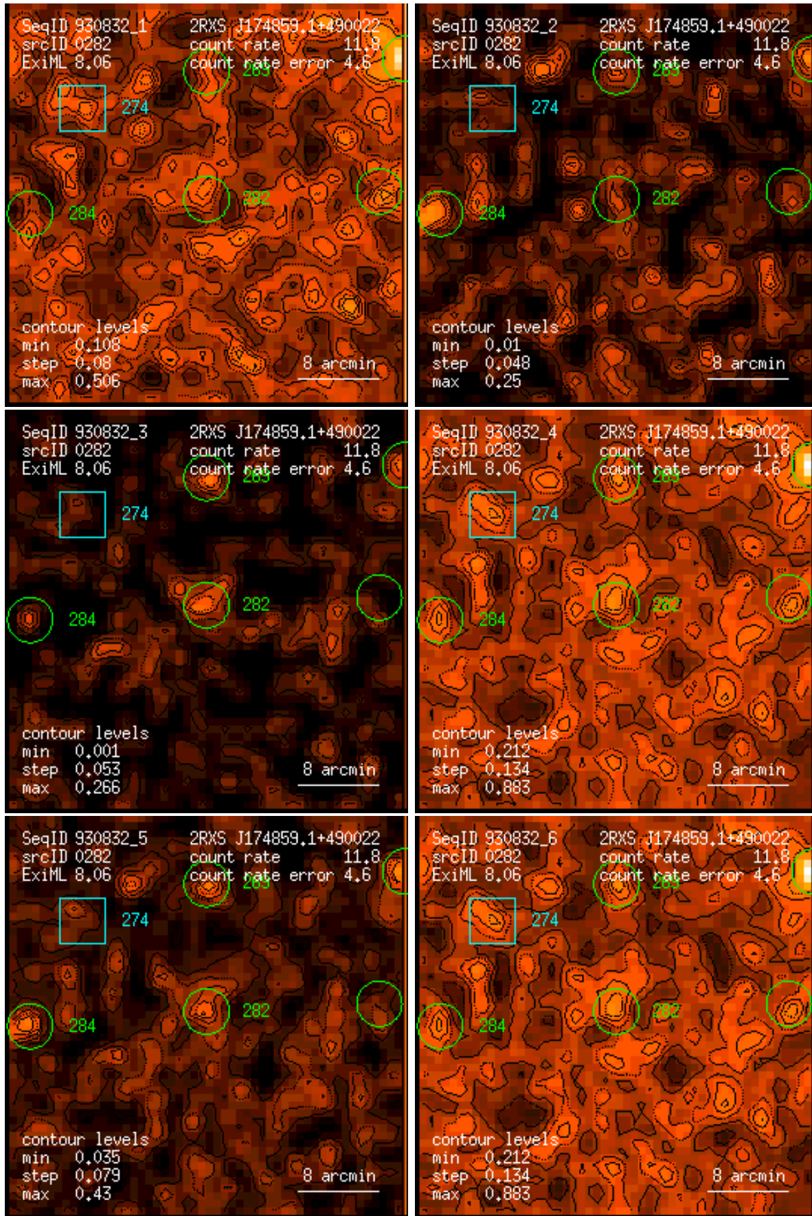
Figure 282: RASS 930832: detection 0282: band rate images, Gaussian filter: (1) PSPC channels 11 – 41, (2) 52 – 90, (3) 91 – 201, (4) 11 – 235, (5) 52 – 201, (6) 11 – 201. Broad band rates in counts/ks. Band rate contour levels in counts/ks/arcmin 2 .
