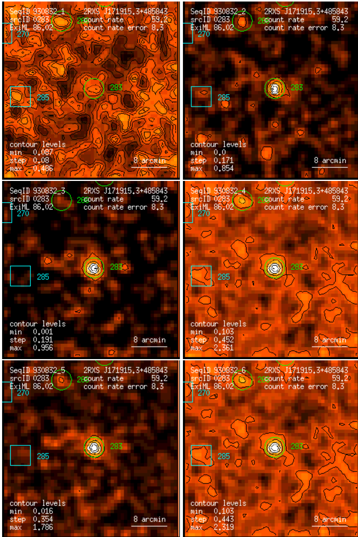
Figure 283: RASS 930832: detection 0283: band rate images, Gaussian filter: (1) PSPC channels 11 – 41, (2) 52 – 90, (3) 91 – 201, (4) 11 – 235, (5) 52 – 201, (6) 11 – 201. Broad band rates in counts/ks. Band rate contour levels in counts/ks/arcmin 2 .
