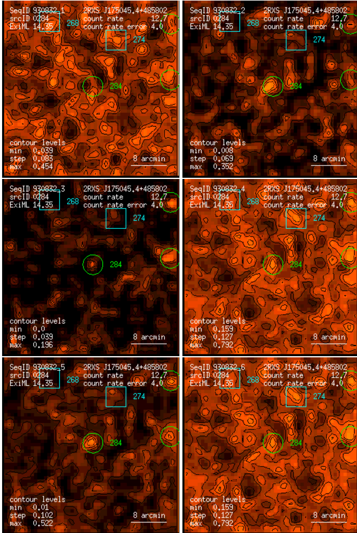
Figure 284: RASS 930832: detection 0284: band rate images, Gaussian filter: (1) PSPC channels 11 – 41, (2) 52 – 90, (3) 91 – 201, (4) 11 – 235, (5) 52 – 201, (6) 11 – 201. Broad band rates in counts/ks. Band rate contour levels in counts/ks/arcmin 2 .
