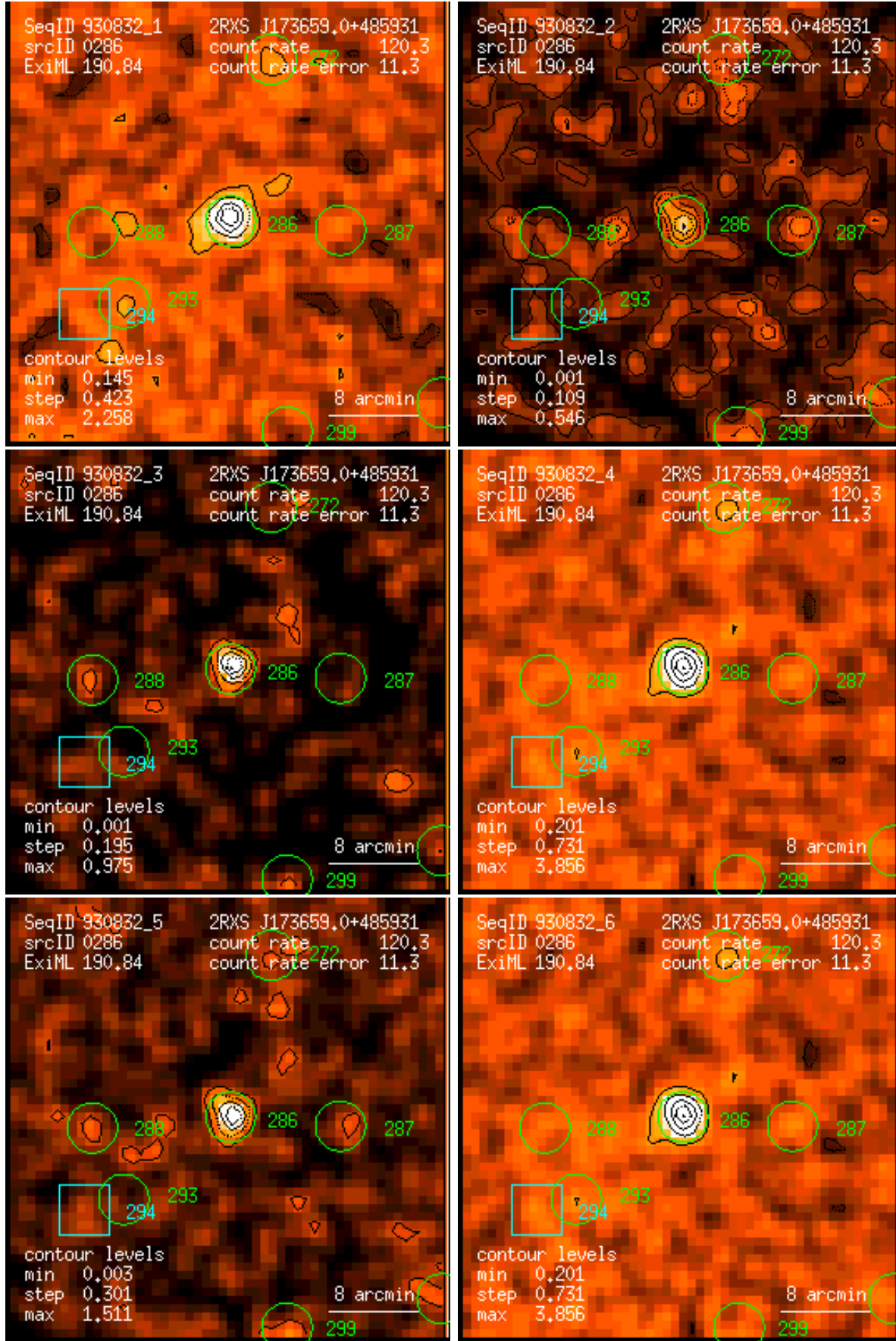
Figure 286: RASS 930832: detection 0286: band rate images, Gaussian filter: (1) PSPC channels 11 – 41, (2) 52 – 90, (3) 91 – 201, (4) 11 – 235, (5) 52 – 201, (6) 11 – 201. Broad band rates in counts/ks. Band rate contour levels in counts/ks/arcmin 2 .
