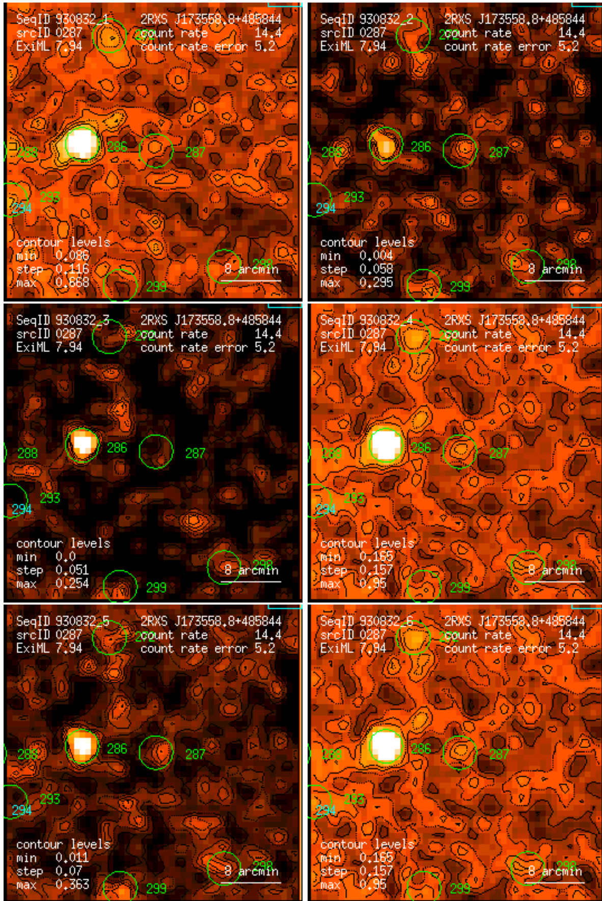
Figure 287: RASS 930832: detection 0287: band rate images, Gaussian filter: (1) PSPC channels 11 – 41, (2) 52 – 90, (3) 91 – 201, (4) 11 – 235, (5) 52 – 201, (6) 11 – 201. Broad band rates in counts/ks. Band rate contour levels in counts/ks/arcmin 2 .
