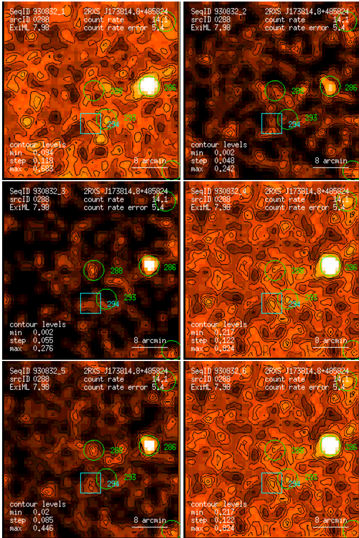
Figure 288: RASS 930832: detection 0288: band rate images, Gaussian filter: (1) PSPC channels 11 – 41, (2) 52 – 90, (3) 91 – 201, (4) 11 – 235, (5) 52 – 201, (6) 11 – 201. Broad band rates in counts/ks. Band rate contour levels in counts/ks/arcmin 2 .
