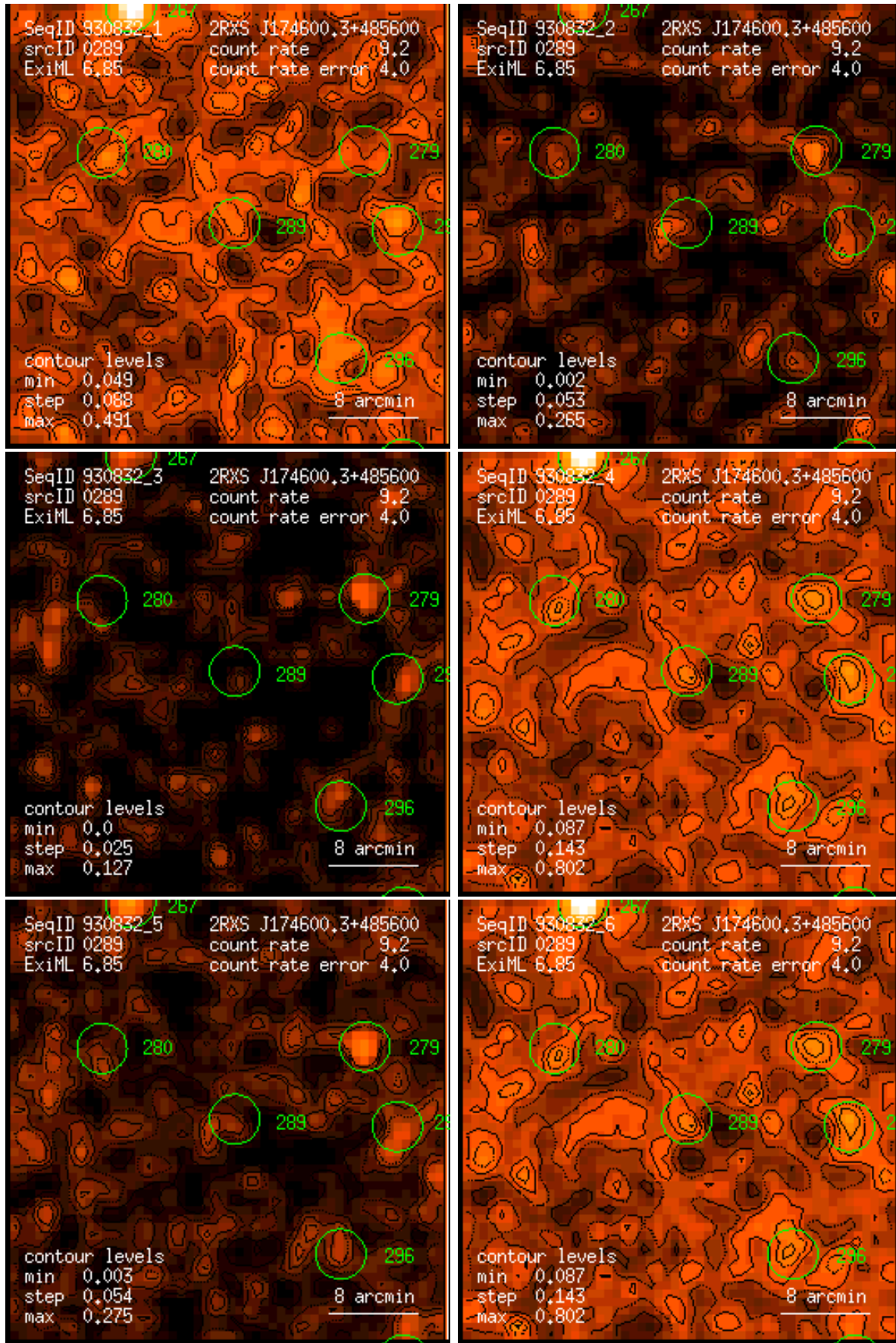
Figure 289: RASS 930832: detection 0289: band rate images, Gaussian filter: (1) PSPC channels 11 – 41, (2) 52 – 90, (3) 91 – 201, (4) 11 – 235, (5) 52 – 201, (6) 11 – 201. Broad band rates in counts/ks. Band rate contour levels in counts/ks/arcmin 2 .
