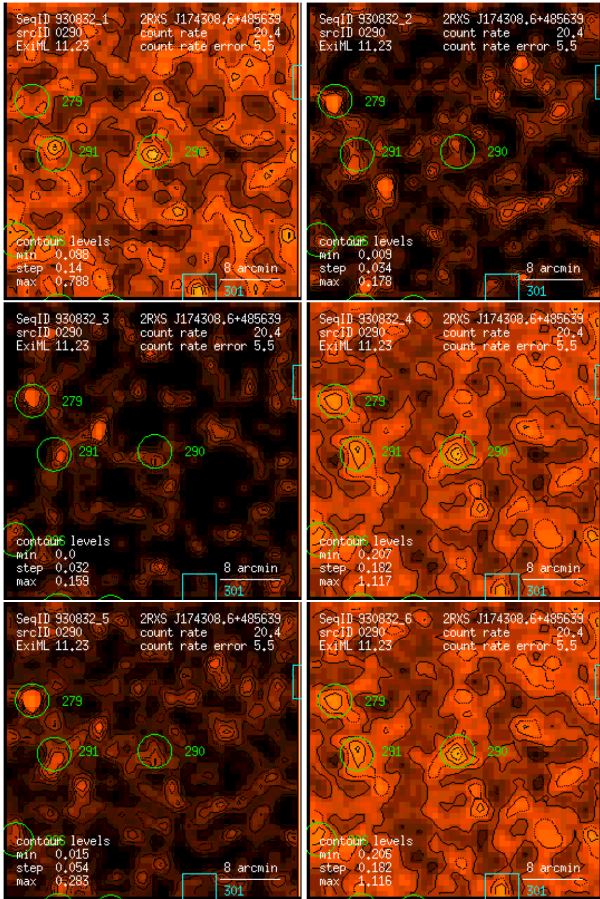
Figure 290: RASS 930832: detection 0290: band rate images, Gaussian filter: (1) PSPC channels 11 – 41, (2) 52 – 90, (3) 91 – 201, (4) 11 – 235, (5) 52 – 201, (6) 11 – 201. Broad band rates in counts/ks. Band rate contour levels in counts/ks/arcmin 2 .
