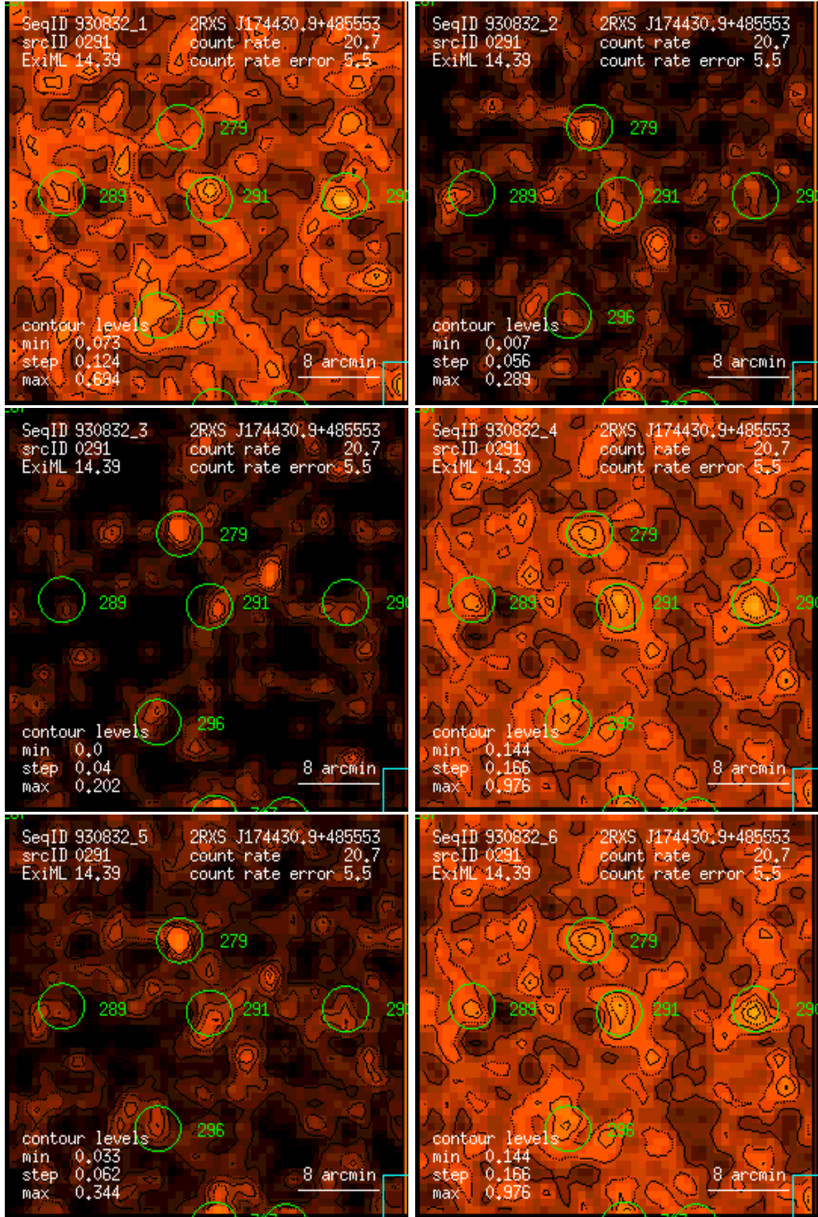
Figure 291: RASS 930832: detection 0291: band rate images, Gaussian filter: (1) PSPC channels 11 – 41, (2) 52 – 90, (3) 91 – 201, (4) 11 – 235, (5) 52 – 201, (6) 11 – 201. Broad band rates in counts/ks. Band rate contour levels in counts/ks/arcmin 2 .
