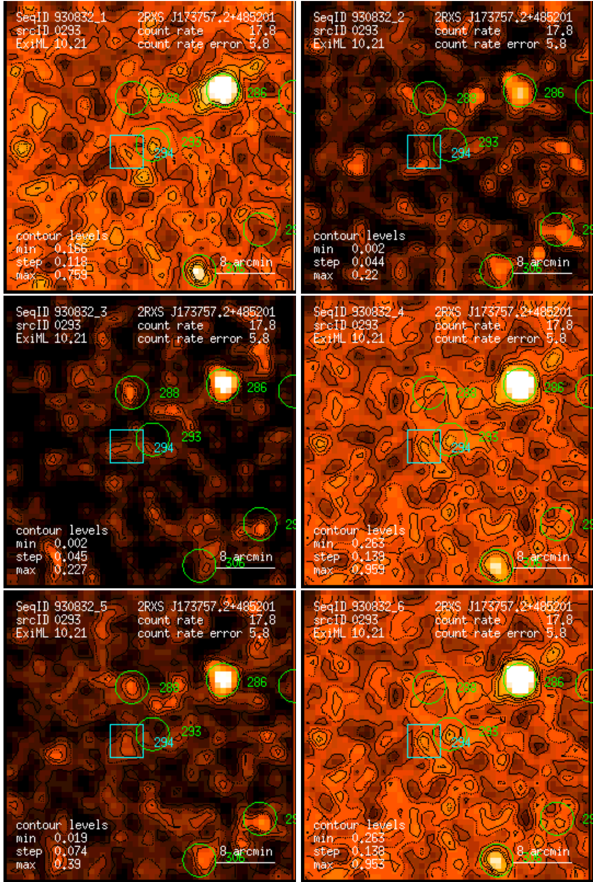
Figure 293: RASS 930832: detection 0293: band rate images, Gaussian filter: (1) PSPC channels 11 – 41, (2) 52 – 90, (3) 91 – 201, (4) 11 – 235, (5) 52 – 201, (6) 11 – 201. Broad band rates in counts/ks. Band rate contour levels in counts/ks/arcmin 2 .
