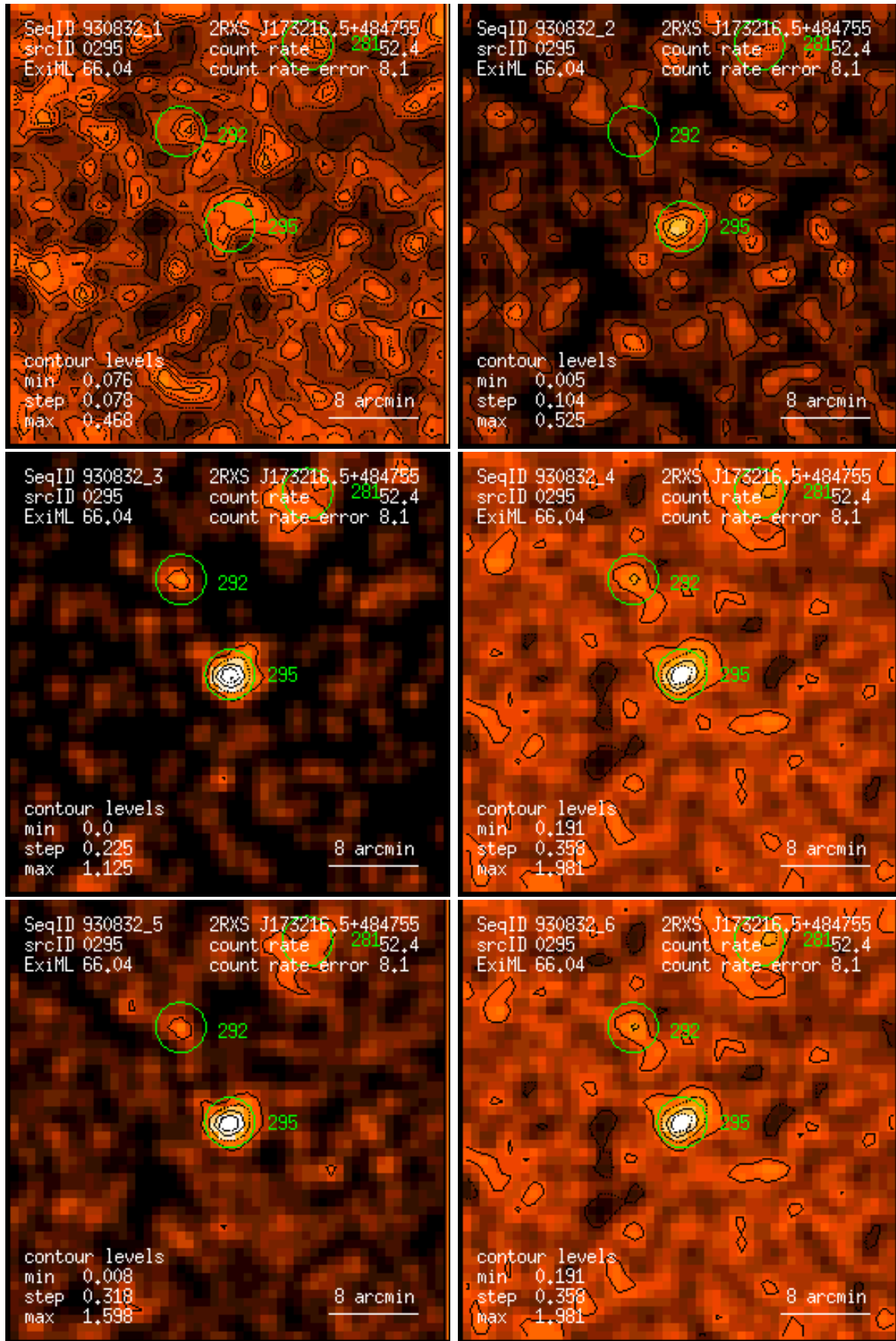
Figure 295: RASS 930832: detection 0295: band rate images, Gaussian filter: (1) PSPC channels 11 – 41, (2) 52 – 90, (3) 91 – 201, (4) 11 – 235, (5) 52 – 201, (6) 11 – 201. Broad band rates in counts/ks. Band rate contour levels in counts/ks/arcmin 2 .
