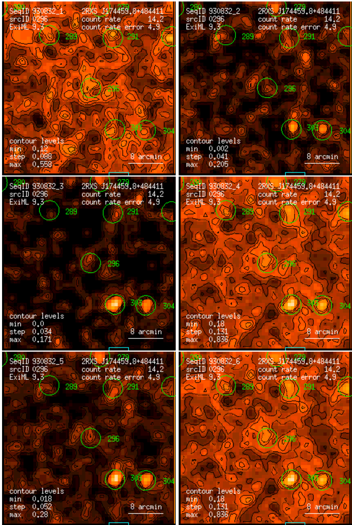
Figure 296: RASS 930832: detection 0296: band rate images, Gaussian filter: (1) PSPC channels 11 – 41, (2) 52 – 90, (3) 91 – 201, (4) 11 – 235, (5) 52 – 201, (6) 11 – 201. Broad band rates in counts/ks. Band rate contour levels in counts/ks/arcmin 2 .
