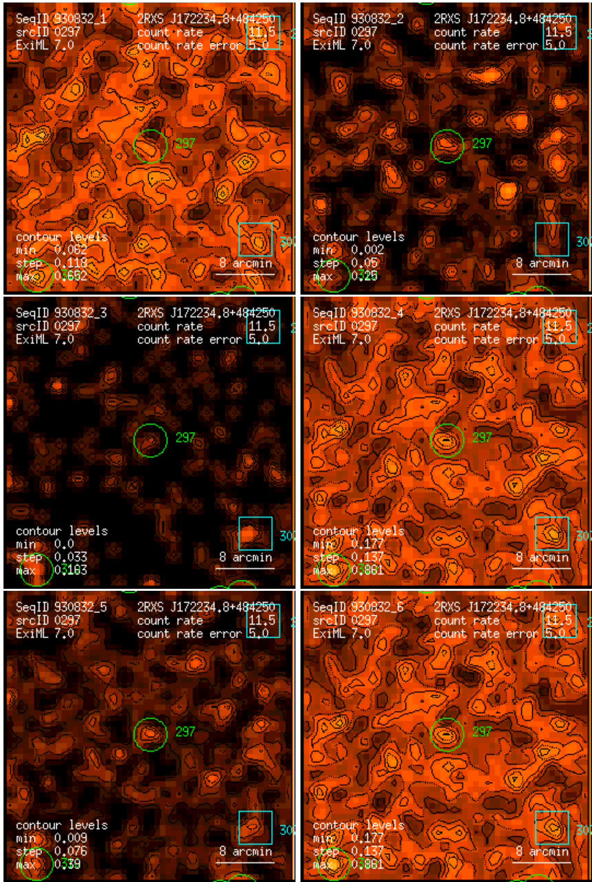
Figure 297: RASS 930832: detection 0297: band rate images, Gaussian filter: (1) PSPC channels 11 – 41, (2) 52 – 90, (3) 91 – 201, (4) 11 – 235, (5) 52 – 201, (6) 11 – 201. Broad band rates in counts/ks. Band rate contour levels in counts/ks/arcmin 2 .
