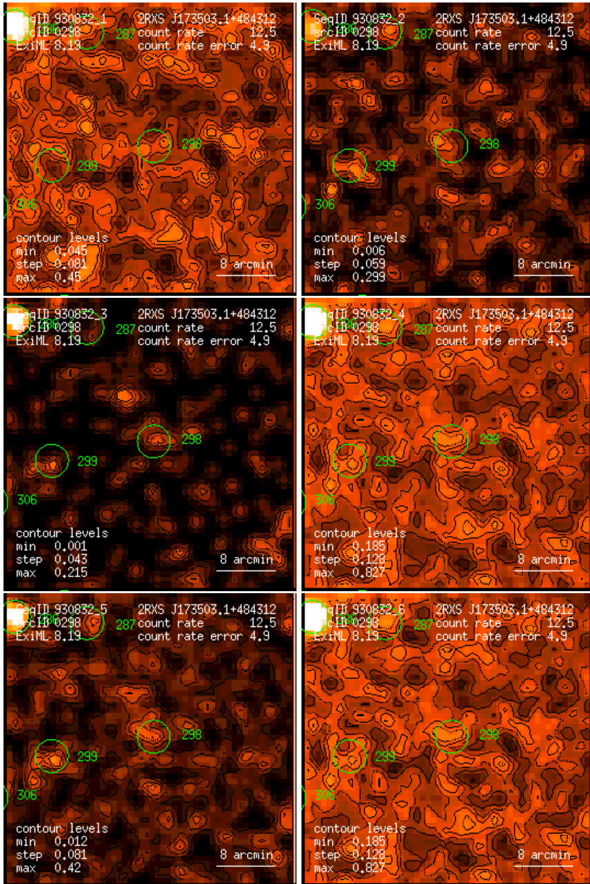
Figure 298: RASS 930832: detection 0298: band rate images, Gaussian filter: (1) PSPC channels 11 – 41, (2) 52 – 90, (3) 91 – 201, (4) 11 – 235, (5) 52 – 201, (6) 11 – 201. Broad band rates in counts/ks. Band rate contour levels in counts/ks/arcmin 2 .
