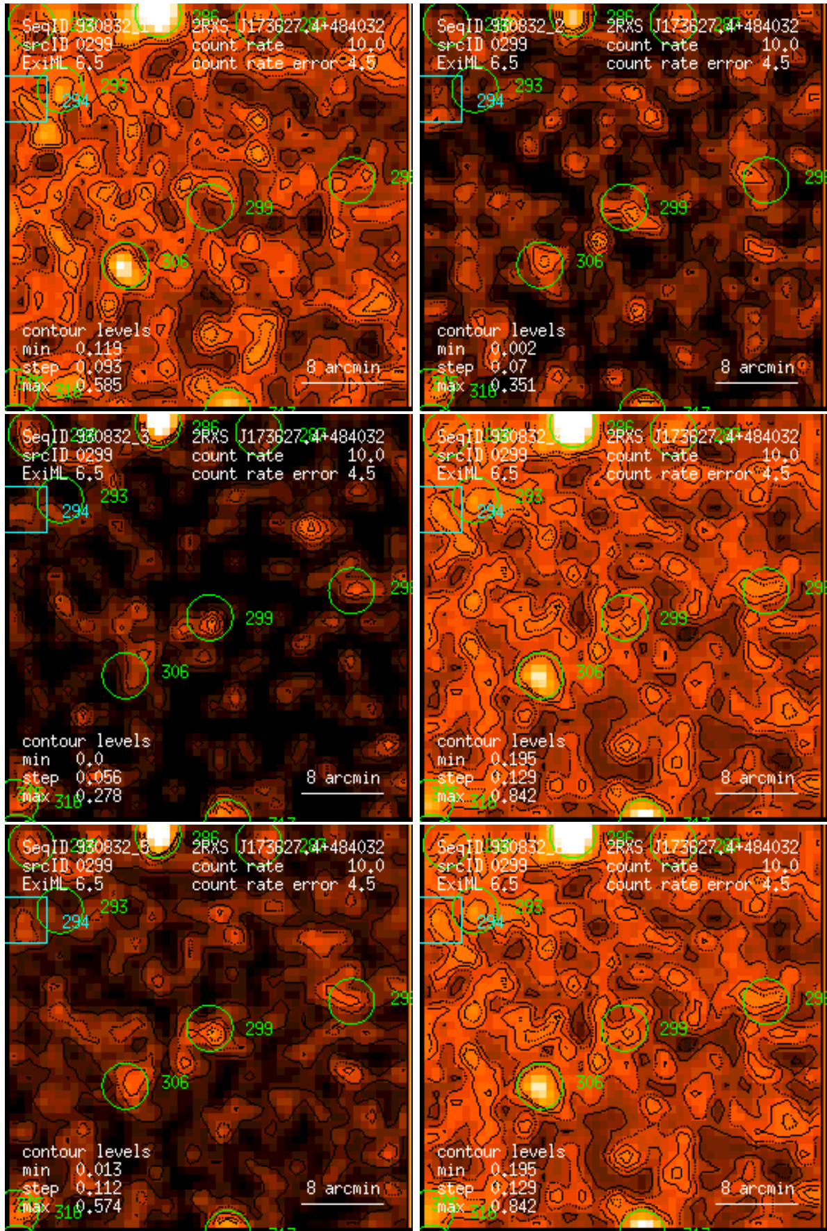
Figure 299: RASS 930832: detection 0299: band rate images, Gaussian filter: (1) PSPC channels 11 – 41, (2) 52 – 90, (3) 91 – 201, (4) 11 – 235, (5) 52 – 201, (6) 11 – 201. Broad band rates in counts/ks. Band rate contour levels in counts/ks/arcmin 2 .
