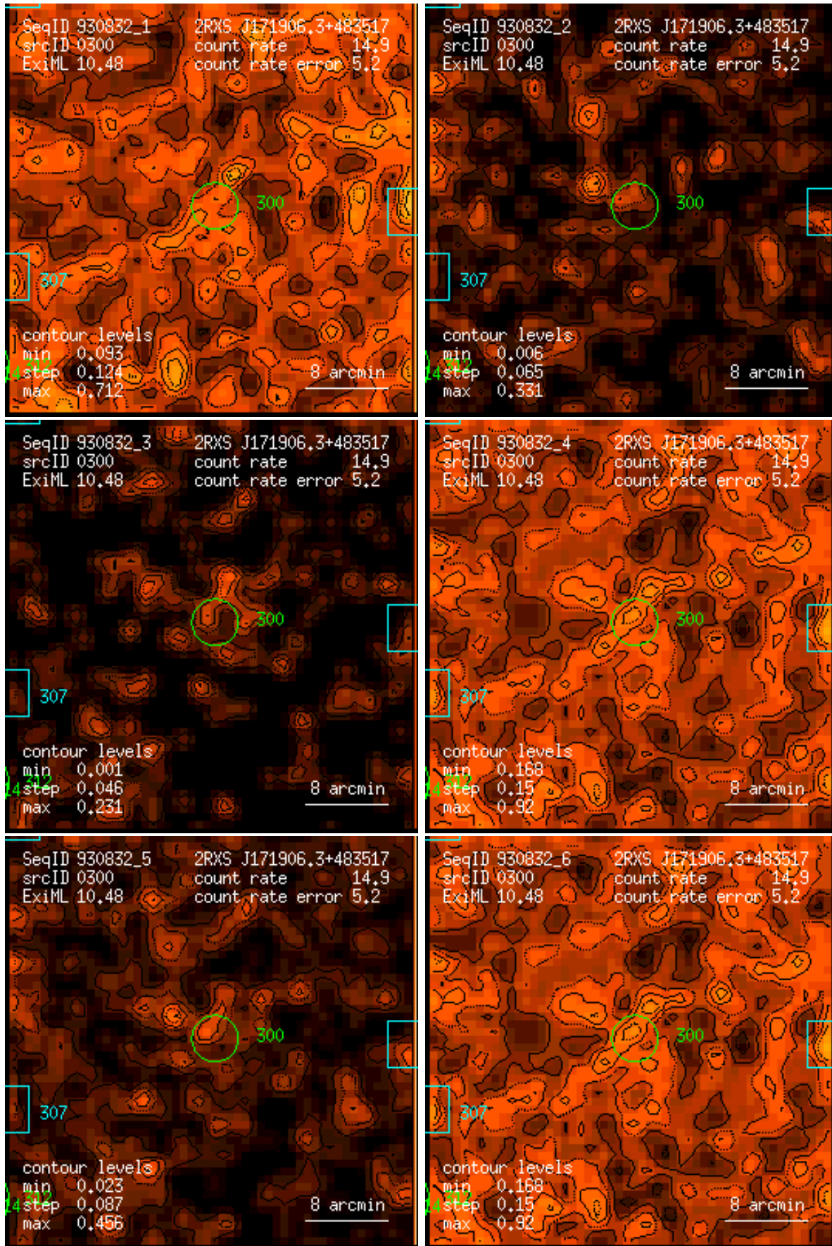
Figure 300: RASS 930832: detection 0300: band rate images, Gaussian filter: (1) PSPC channels 11 – 41, (2) 52 – 90, (3) 91 – 201, (4) 11 – 235, (5) 52 – 201, (6) 11 – 201. Broad band rates in counts/ks. Band rate contour levels in counts/ks/arcmin 2 .
