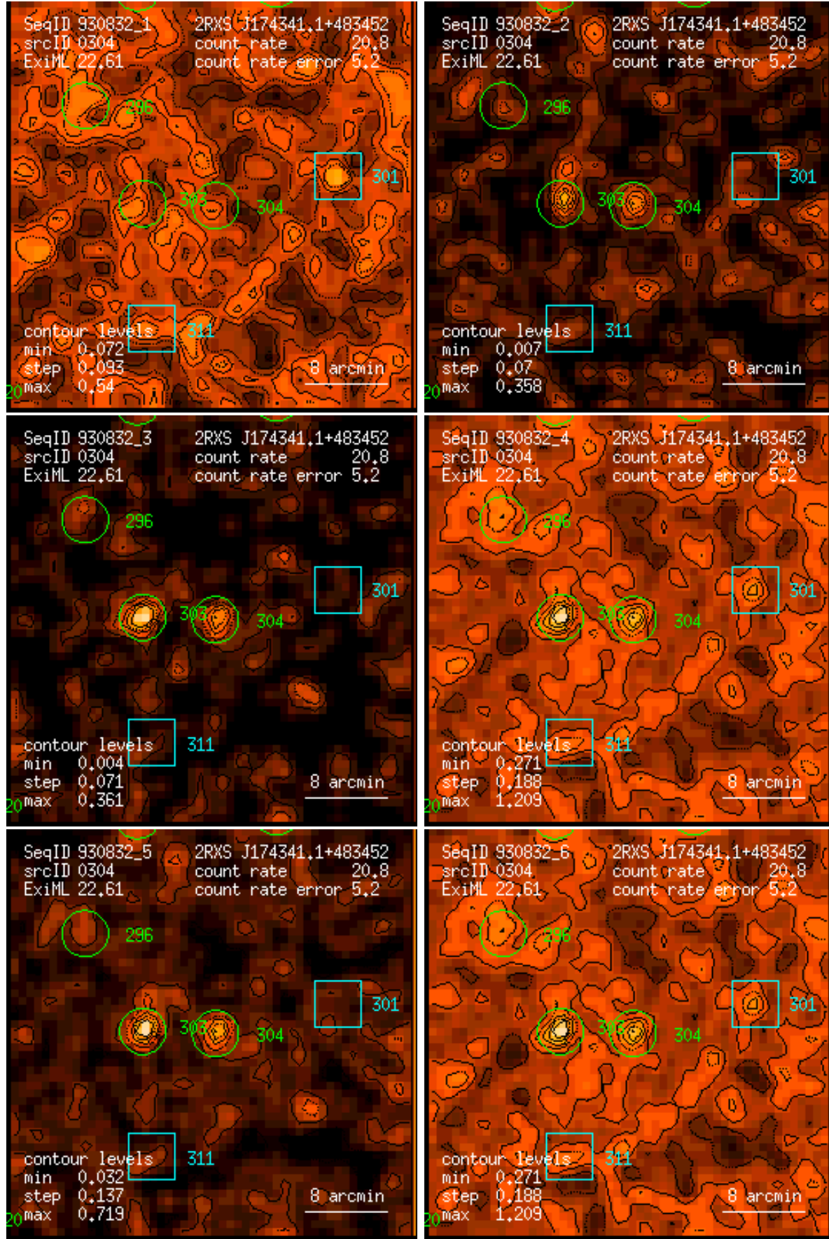
Figure 304: RASS 930832: detection 0304: band rate images, Gaussian filter: (1) PSPC channels 11 – 41, (2) 52 – 90, (3) 91 – 201, (4) 11 – 235, (5) 52 – 201, (6) 11 – 201. Broad band rates in counts/ks. Band rate contour levels in counts/ks/arcmin 2 .
