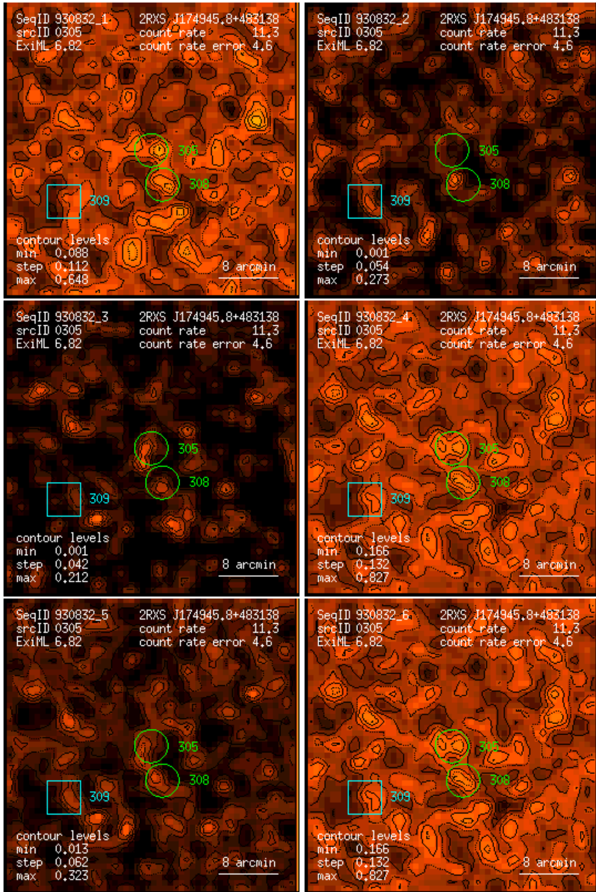
Figure 305: RASS 930832: detection 0305: band rate images, Gaussian filter: (1) PSPC channels 11 – 41, (2) 52 – 90, (3) 91 – 201, (4) 11 – 235, (5) 52 – 201, (6) 11 – 201. Broad band rates in counts/ks. Band rate contour levels in counts/ks/arcmin 2 .
