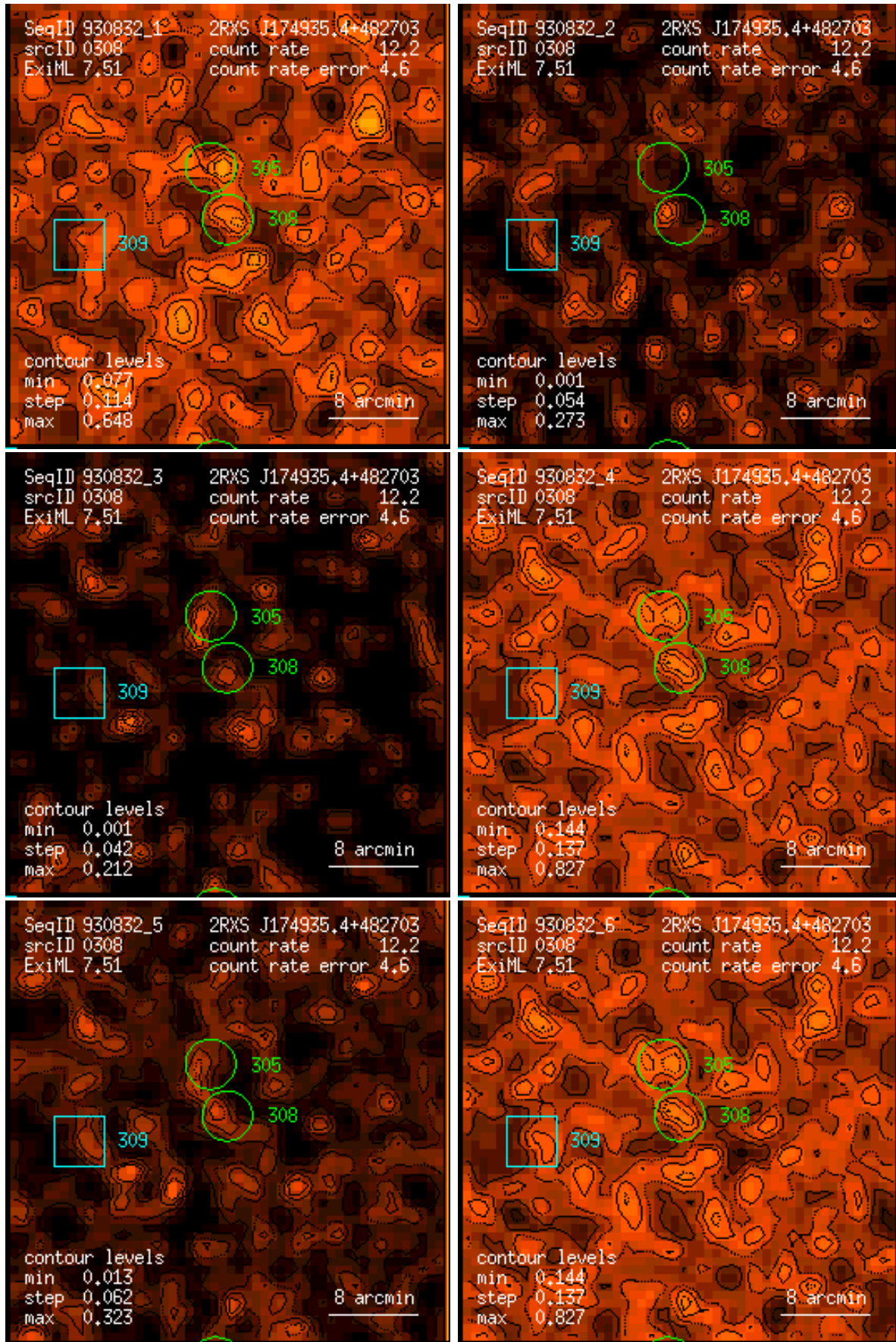
Figure 308: RASS 930832: detection 0308: band rate images, Gaussian filter: (1) PSPC channels 11 – 41, (2) 52 – 90, (3) 91 – 201, (4) 11 – 235, (5) 52 – 201, (6) 11 – 201. Broad band rates in counts/ks. Band rate contour levels in counts/ks/arcmin 2 .
