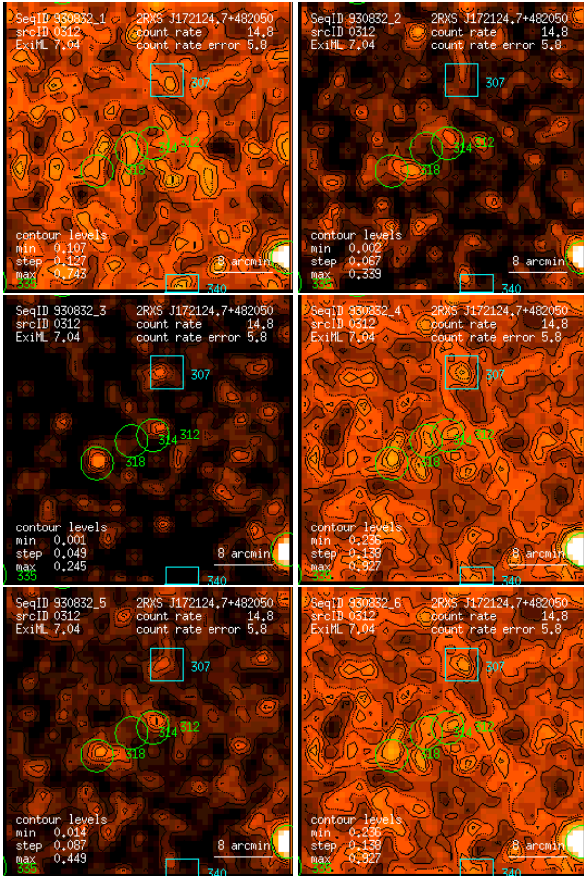
Figure 312: RASS 930832: detection 0312: band rate images, Gaussian filter: (1) PSPC channels 11 – 41, (2) 52 – 90, (3) 91 – 201, (4) 11 – 235, (5) 52 – 201, (6) 11 – 201. Broad band rates in counts/ks. Band rate contour levels in counts/ks/arcmin 2 .
