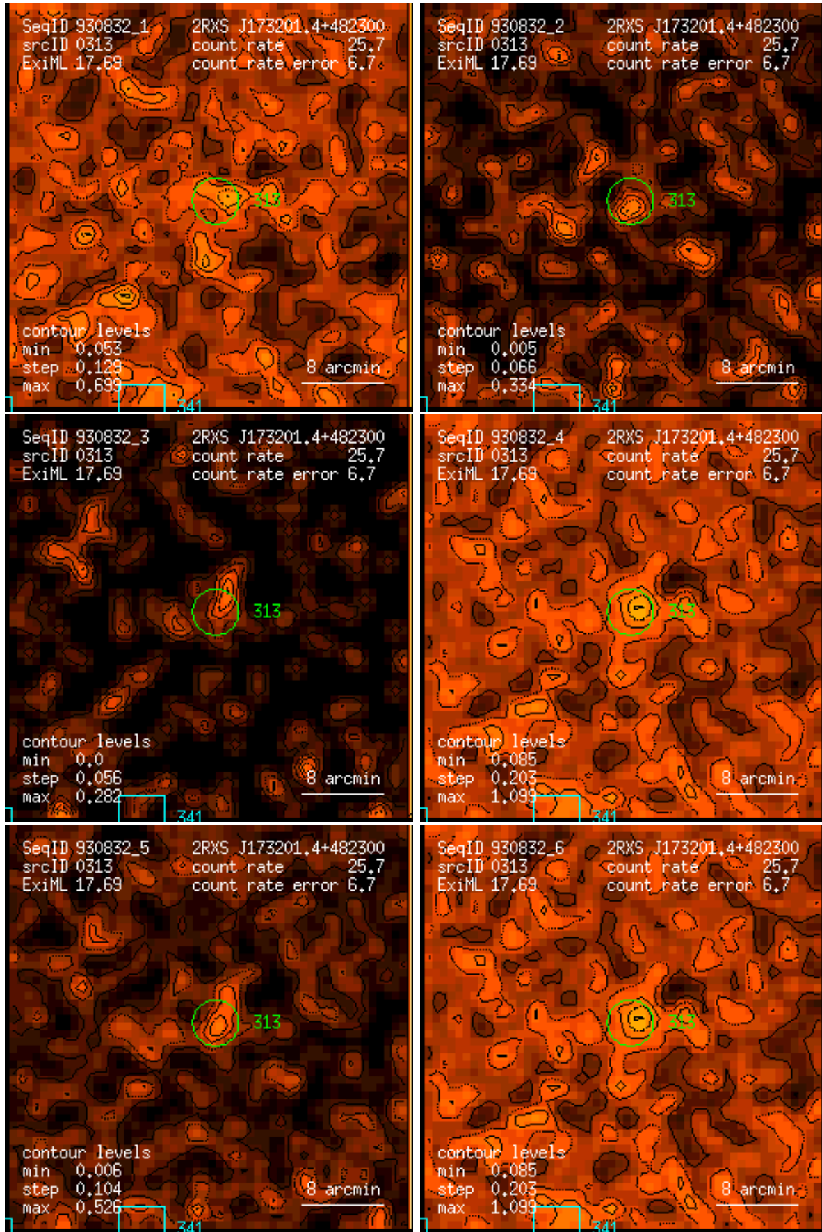
Figure 313: RASS 930832: detection 0313: band rate images, Gaussian filter: (1) PSPC channels 11 – 41, (2) 52 – 90, (3) 91 – 201, (4) 11 – 235, (5) 52 – 201, (6) 11 – 201. Broad band rates in counts/ks. Band rate contour levels in counts/ks/arcmin 2 .
