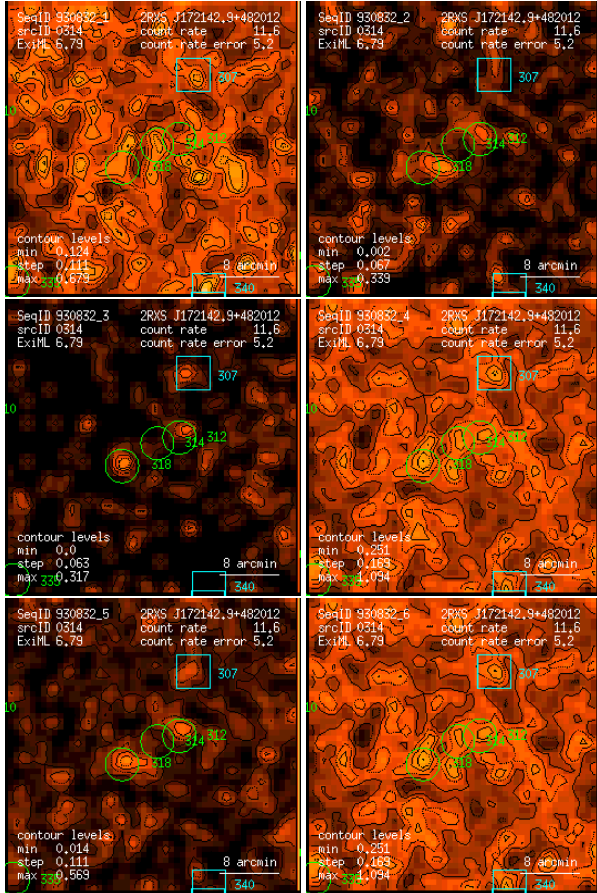
Figure 314: RASS 930832: detection 0314: band rate images, Gaussian filter: (1) PSPC channels 11 – 41, (2) 52 – 90, (3) 91 – 201, (4) 11 – 235, (5) 52 – 201, (6) 11 – 201. Broad band rates in counts/ks. Band rate contour levels in counts/ks/arcmin 2 .
