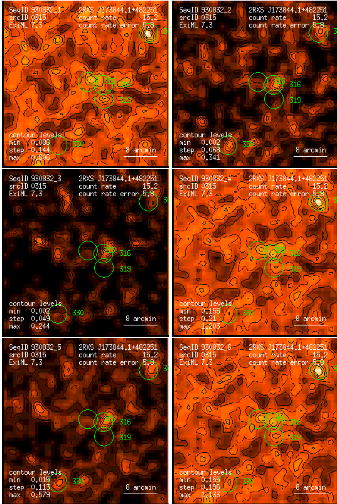
Figure 315: RASS 930832: detection 0315: band rate images, Gaussian filter: (1) PSPC channels 11 – 41, (2) 52 – 90, (3) 91 – 201, (4) 11 – 235, (5) 52 – 201, (6) 11 – 201. Broad band rates in counts/ks. Band rate contour levels in counts/ks/arcmin 2 .
