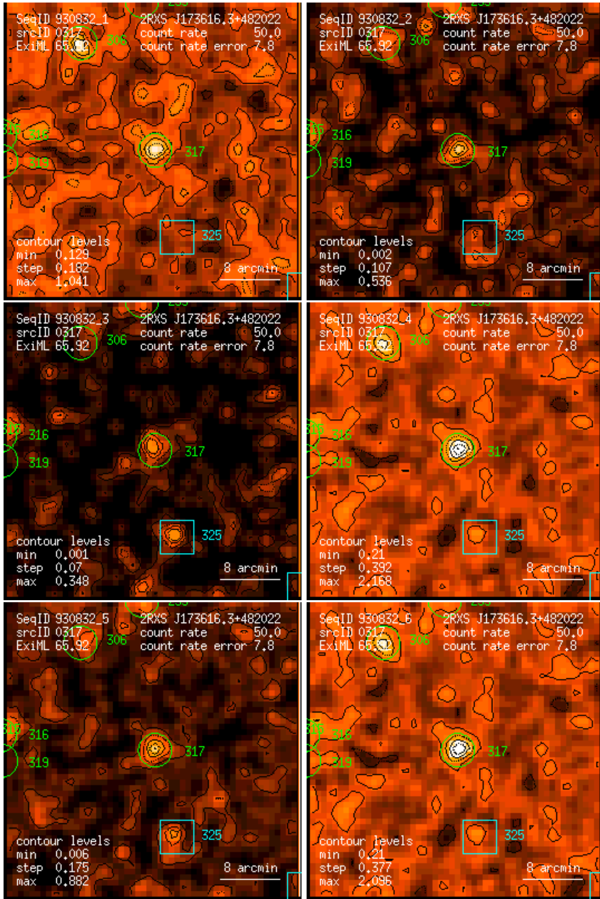
Figure 317: RASS 930832: detection 0317: band rate images, Gaussian filter: (1) PSPC channels 11 – 41, (2) 52 – 90, (3) 91 – 201, (4) 11 – 235, (5) 52 – 201, (6) 11 – 201. Broad band rates in counts/ks. Band rate contour levels in counts/ks/arcmin 2 .
