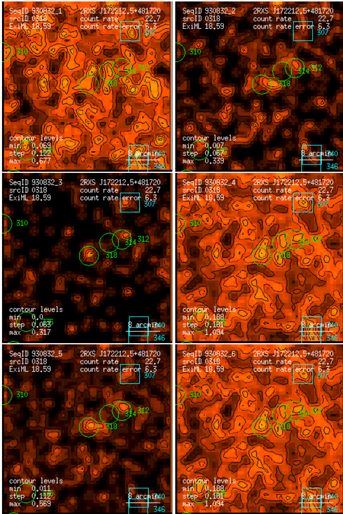
Figure 318: RASS 930832: detection 0318: band rate images, Gaussian filter: (1) PSPC channels 11 – 41, (2) 52 – 90, (3) 91 – 201, (4) 11 – 235, (5) 52 – 201, (6) 11 – 201. Broad band rates in counts/ks. Band rate contour levels in counts/ks/arcmin 2 .
