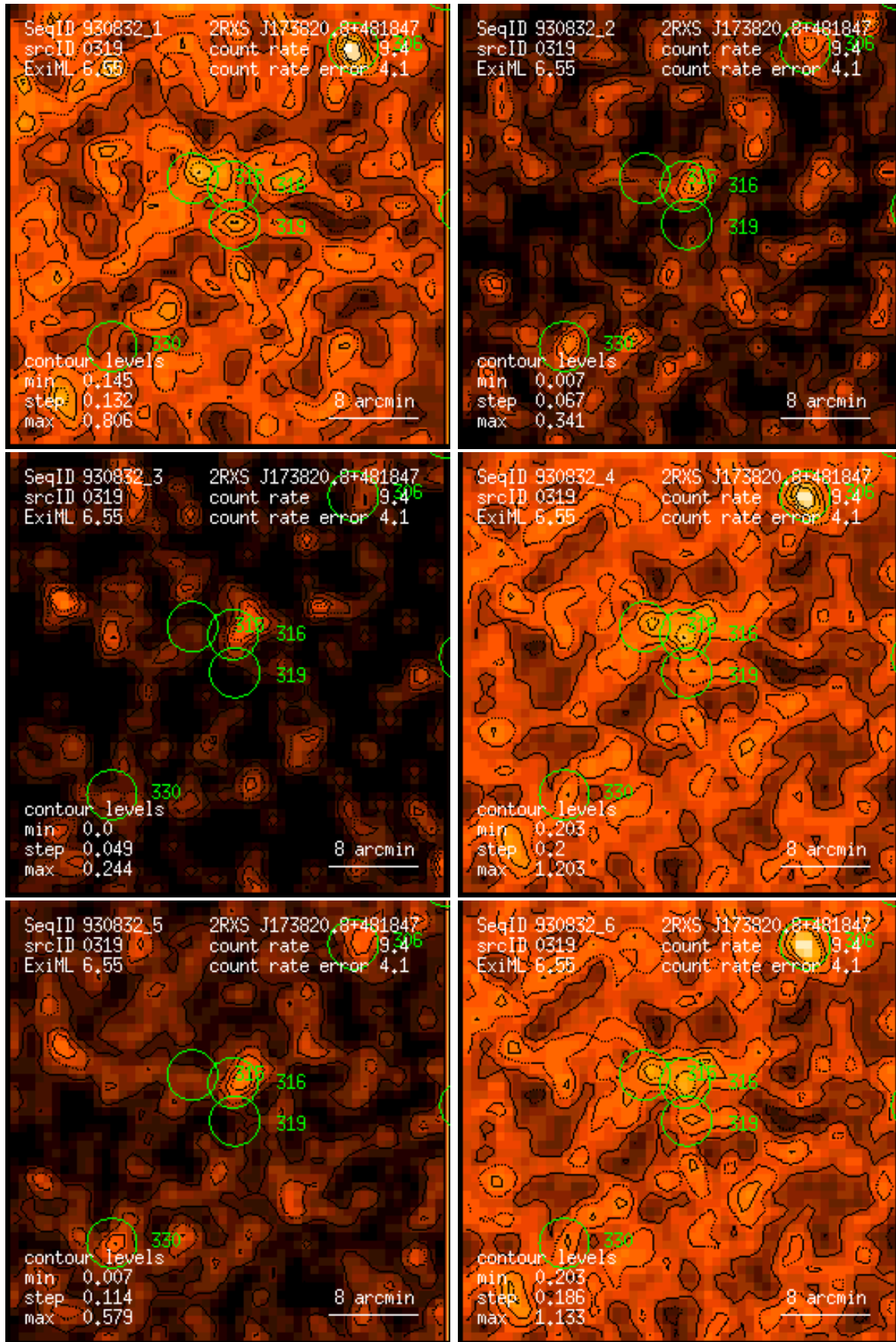
Figure 319: RASS 930832: detection 0319: band rate images, Gaussian filter: (1) PSPC channels 11 – 41, (2) 52 – 90, (3) 91 – 201, (4) 11 – 235, (5) 52 – 201, (6) 11 – 201. Broad band rates in counts/ks. Band rate contour levels in counts/ks/arcmin 2 .
