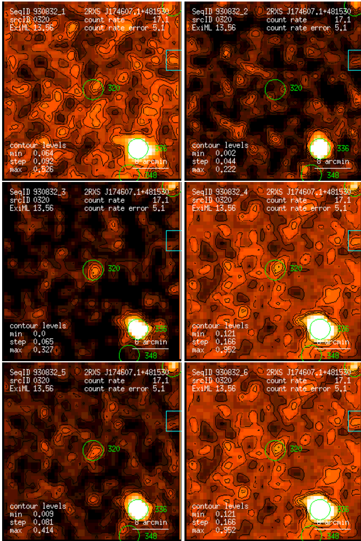
Figure 320: RASS 930832: detection 0320: band rate images, Gaussian filter: (1) PSPC channels 11 – 41, (2) 52 – 90, (3) 91 – 201, (4) 11 – 235, (5) 52 – 201, (6) 11 – 201. Broad band rates in counts/ks. Band rate contour levels in counts/ks/arcmin 2 .
