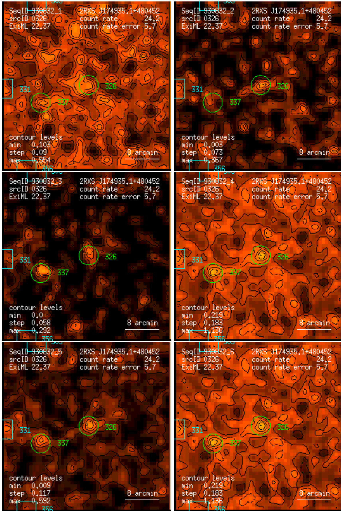
Figure 326: RASS 930832: detection 0326: band rate images, Gaussian filter: (1) PSPC channels 11 – 41, (2) 52 – 90, (3) 91 – 201, (4) 11 – 235, (5) 52 – 201, (6) 11 – 201. Broad band rates in counts/ks. Band rate contour levels in counts/ks/arcmin 2 .
