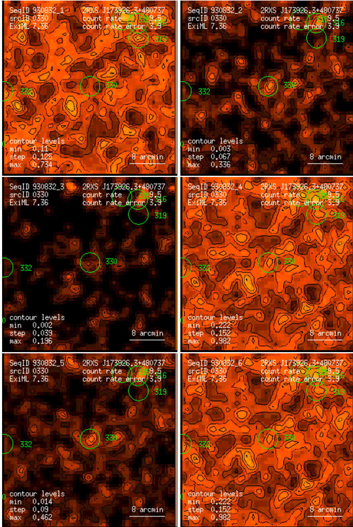
Figure 330: RASS 930832: detection 0330: band rate images, Gaussian filter: (1) PSPC channels 11 – 41, (2) 52 – 90, (3) 91 – 201, (4) 11 – 235, (5) 52 – 201, (6) 11 – 201. Broad band rates in counts/ks. Band rate contour levels in counts/ks/arcmin 2 .
