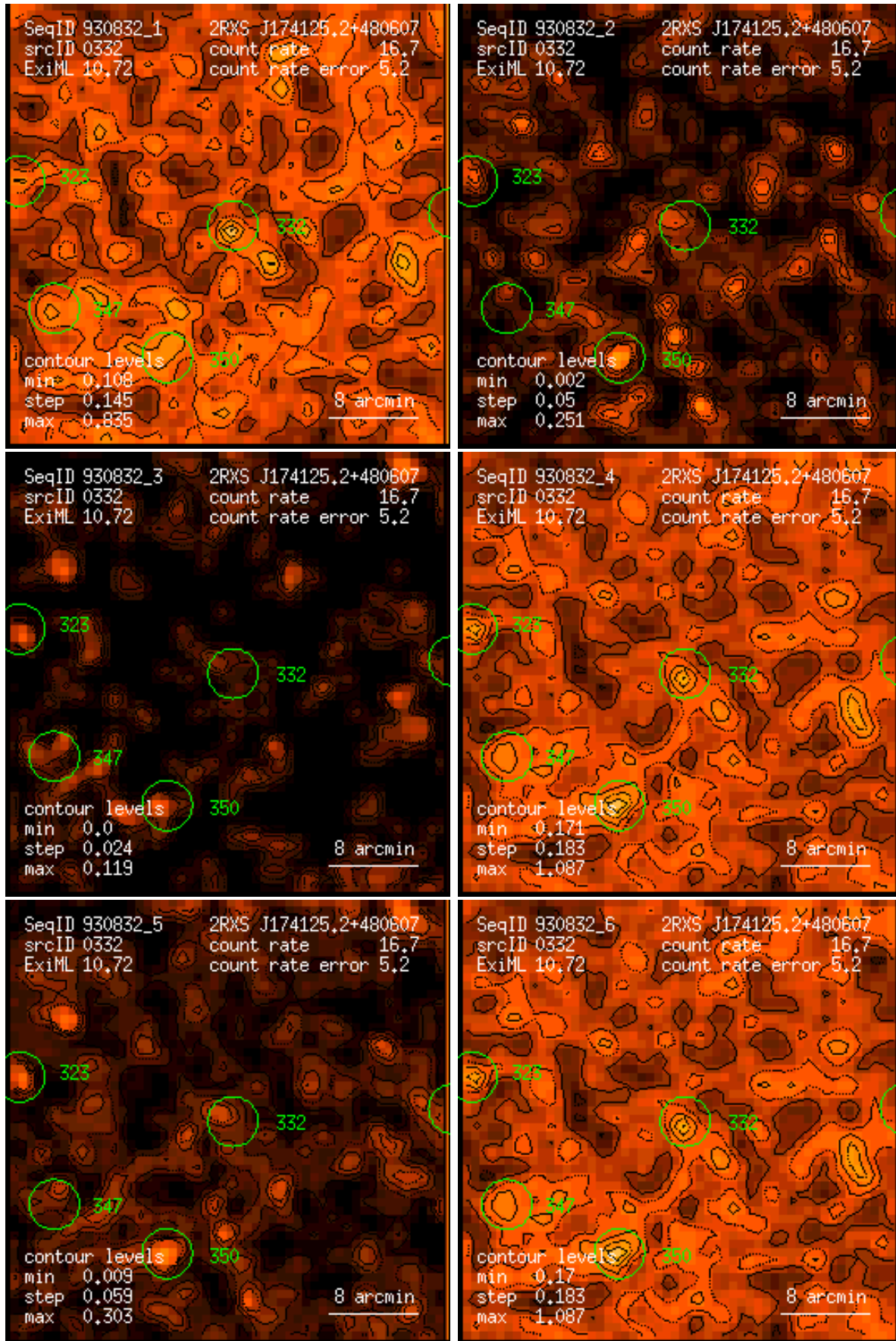
Figure 332: RASS 930832: detection 0332: band rate images, Gaussian filter: (1) PSPC channels 11 – 41, (2) 52 – 90, (3) 91 – 201, (4) 11 – 235, (5) 52 – 201, (6) 11 – 201. Broad band rates in counts/ks. Band rate contour levels in counts/ks/arcmin 2 .
