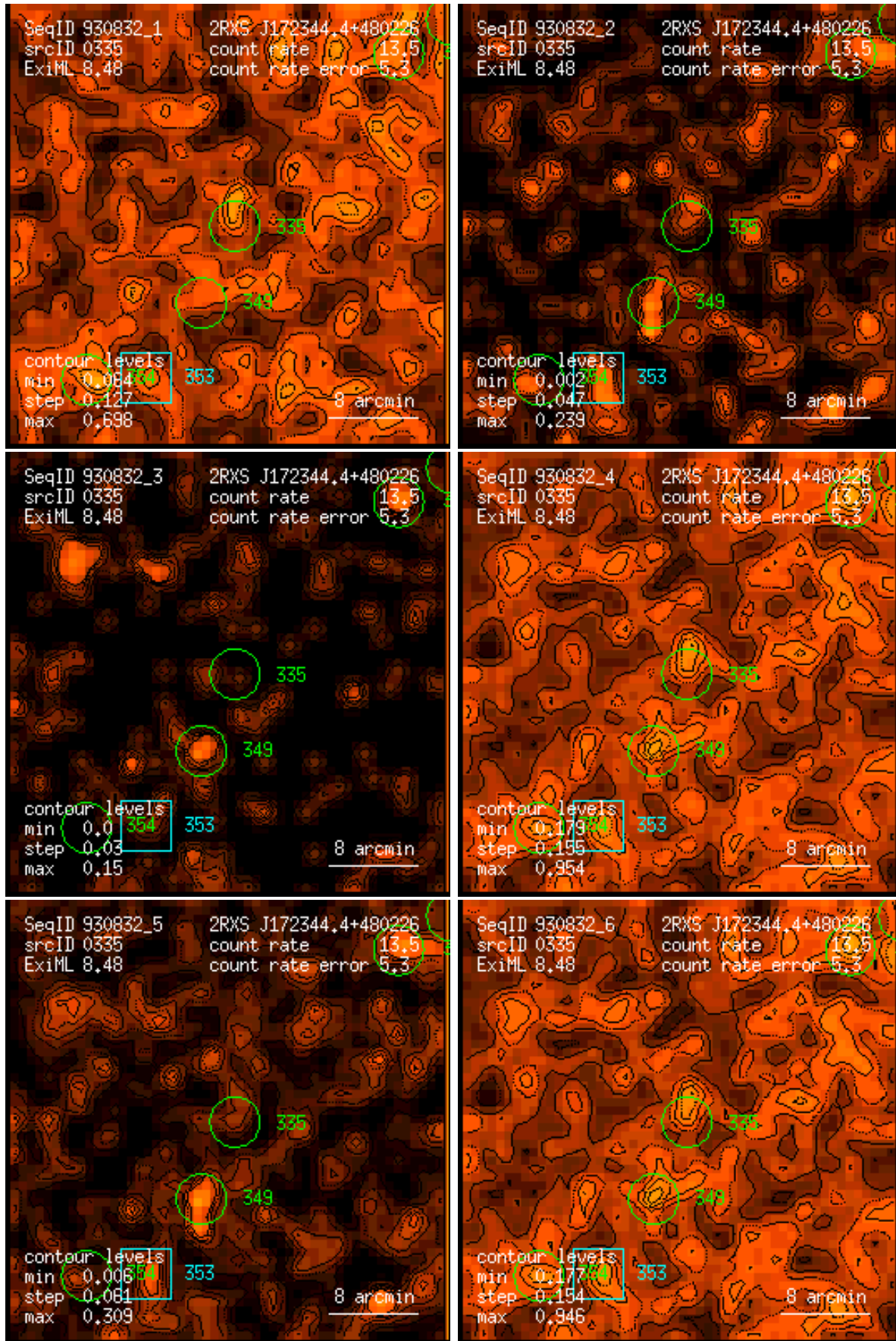
Figure 335: RASS 930832: detection 0335: band rate images, Gaussian filter: (1) PSPC channels 11 – 41, (2) 52 – 90, (3) 91 – 201, (4) 11 – 235, (5) 52 – 201, (6) 11 – 201. Broad band rates in counts/ks. Band rate contour levels in counts/ks/arcmin 2 .
