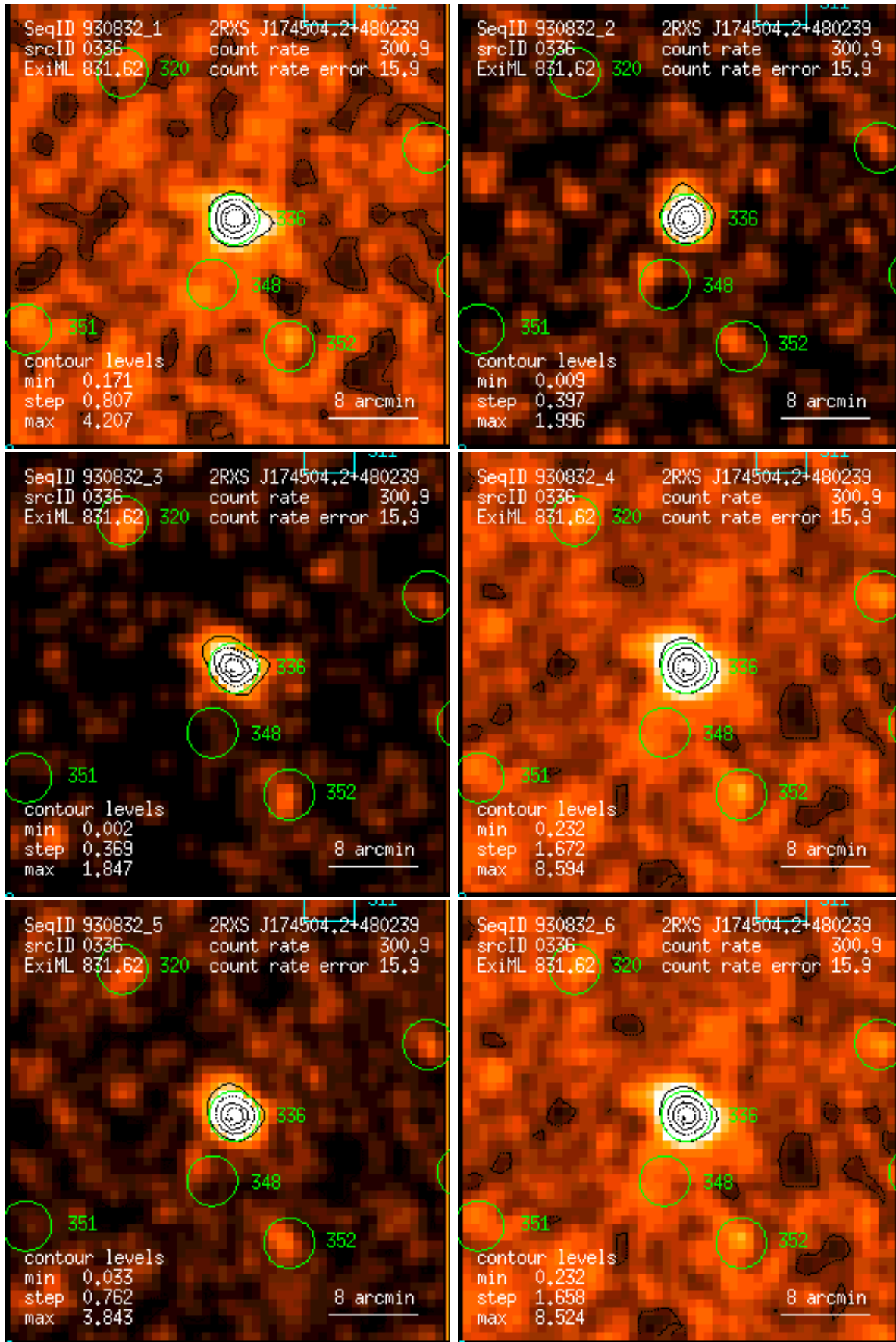
Figure 336: RASS 930832: detection 0336: band rate images, Gaussian filter: (1) PSPC channels 11 – 41, (2) 52 – 90, (3) 91 – 201, (4) 11 – 235, (5) 52 – 201, (6) 11 – 201. Broad band rates in counts/ks. Band rate contour levels in counts/ks/arcmin 2 .
