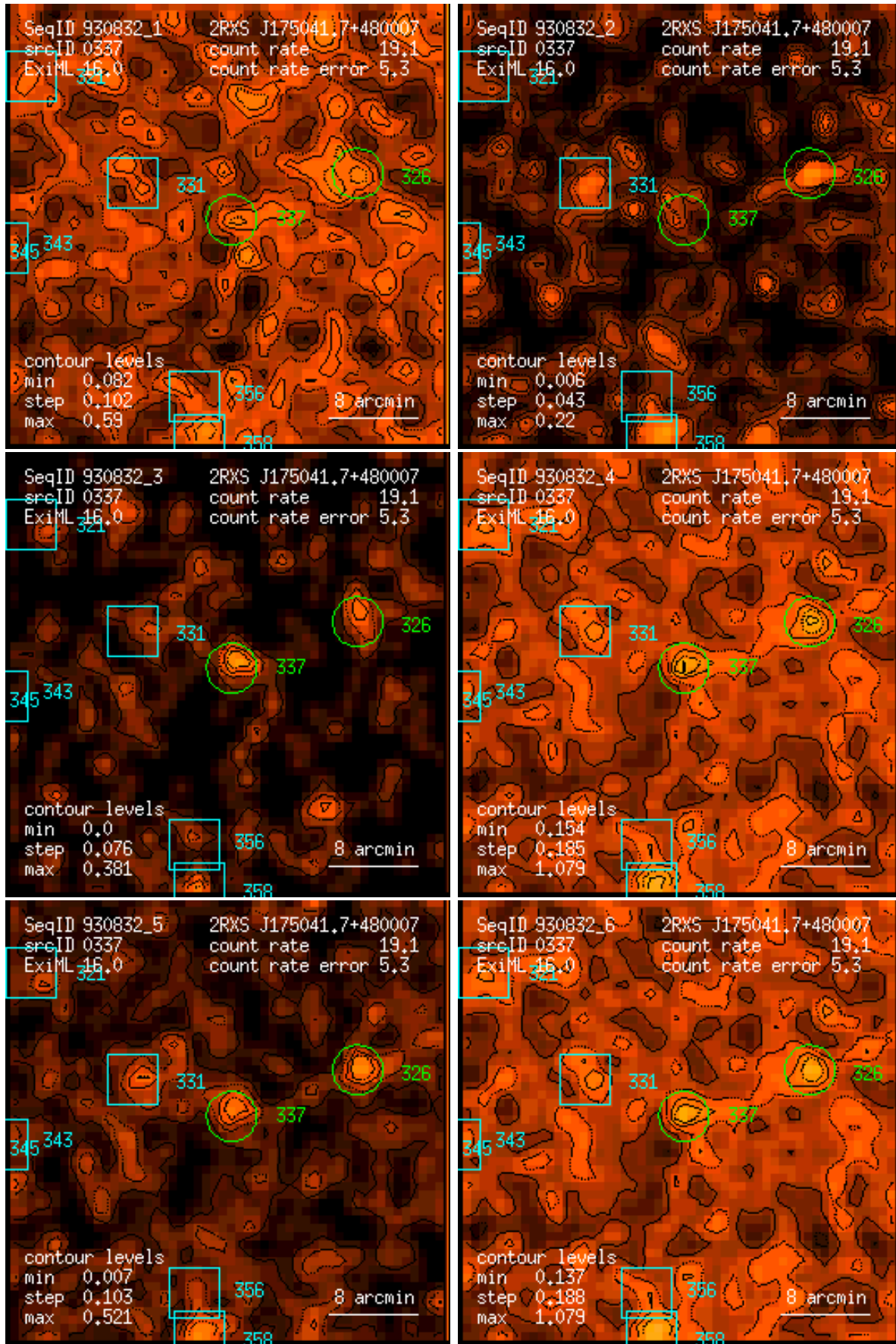
Figure 337: RASS 930832: detection 0337: band rate images, Gaussian filter: (1) PSPC channels 11 – 41, (2) 52 – 90, (3) 91 – 201, (4) 11 – 235, (5) 52 – 201, (6) 11 – 201. Broad band rates in counts/ks. Band rate contour levels in counts/ks/arcmin 2 .
