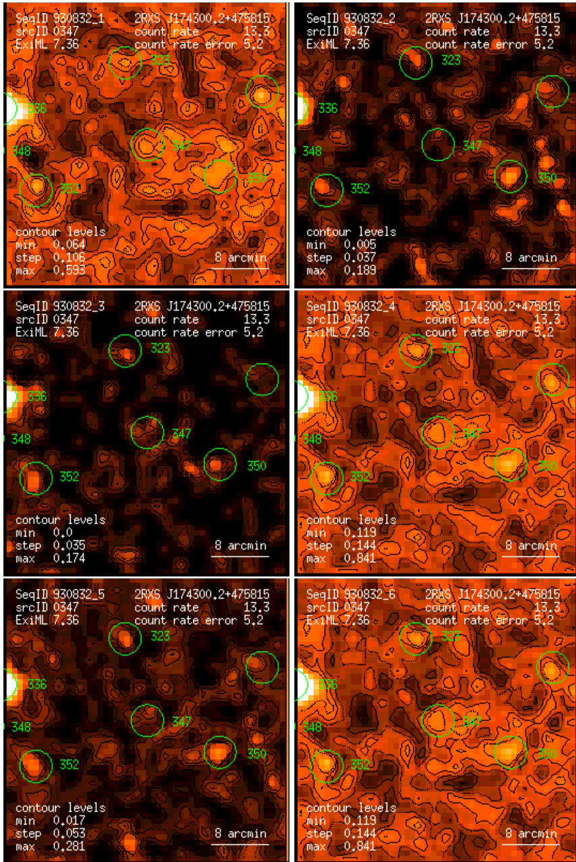
Figure 347: RASS 930832: detection 0347: band rate images, Gaussian filter: (1) PSPC channels 11 – 41, (2) 52 – 90, (3) 91 – 201, (4) 11 – 235, (5) 52 – 201, (6) 11 – 201. Broad band rates in counts/ks. Band rate contour levels in counts/ks/arcmin 2 .
